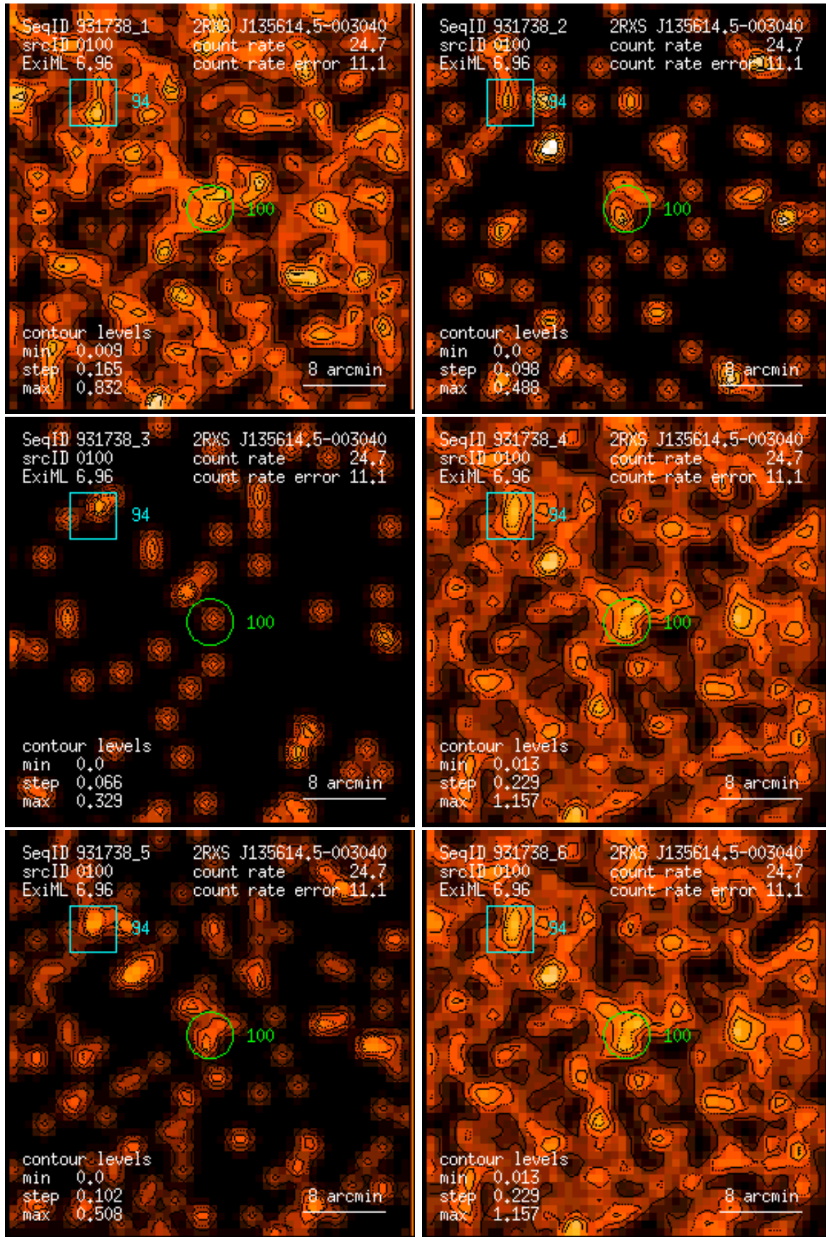
Figure 100: RASS 931738: detection 0100: band rate images, Gaussian filter: (1) PSPC channels 11 – 41, (2) 52 – 90, (3) 91 – 201, (4) 11 – 235, (5) 52 – 201, (6) 11 – 201. Broad band rates in counts/ks. Band rate contour levels in counts/ks/arcmin 2 .
