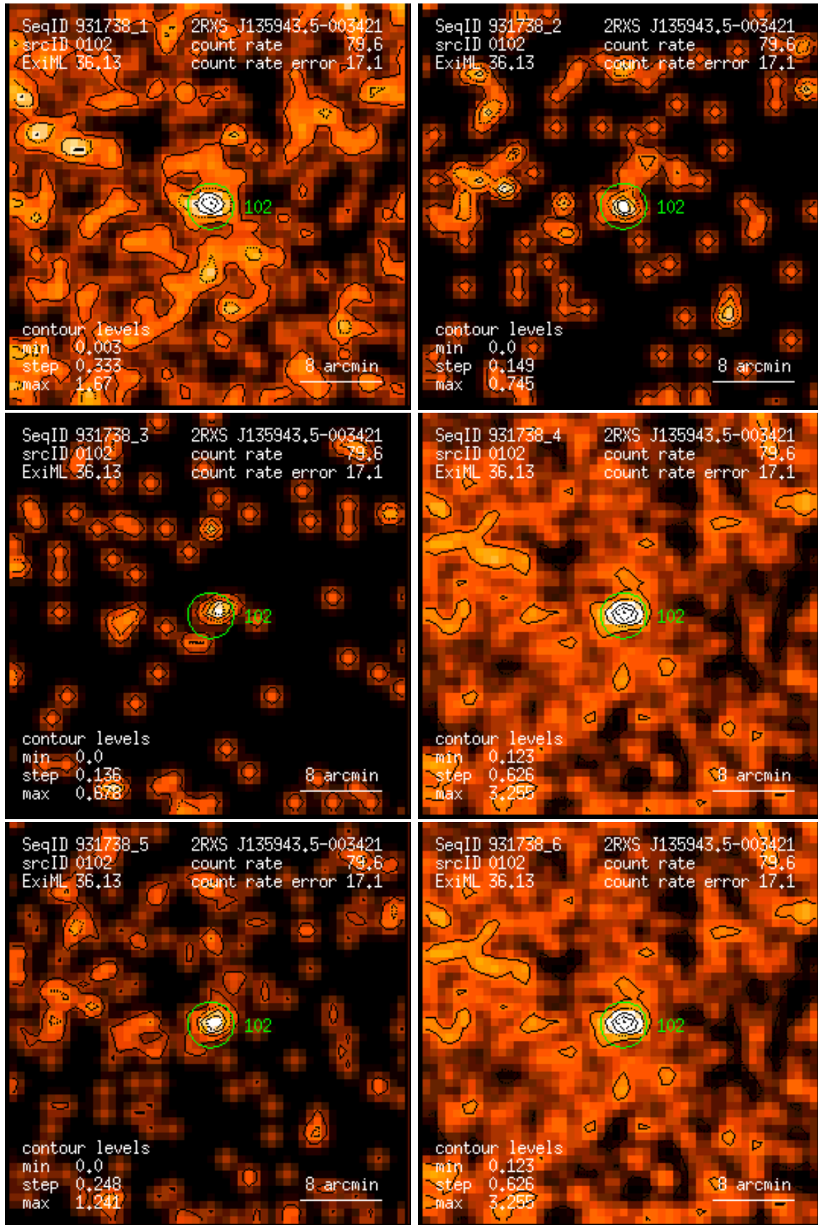
Figure 102: RASS 931738: detection 0102: band rate images, Gaussian filter: (1) PSPC channels 11 – 41, (2) 52 – 90, (3) 91 – 201, (4) 11 – 235, (5) 52 – 201, (6) 11 – 201. Broad band rates in counts/ks. Band rate contour levels in counts/ks/arcmin 2 .
