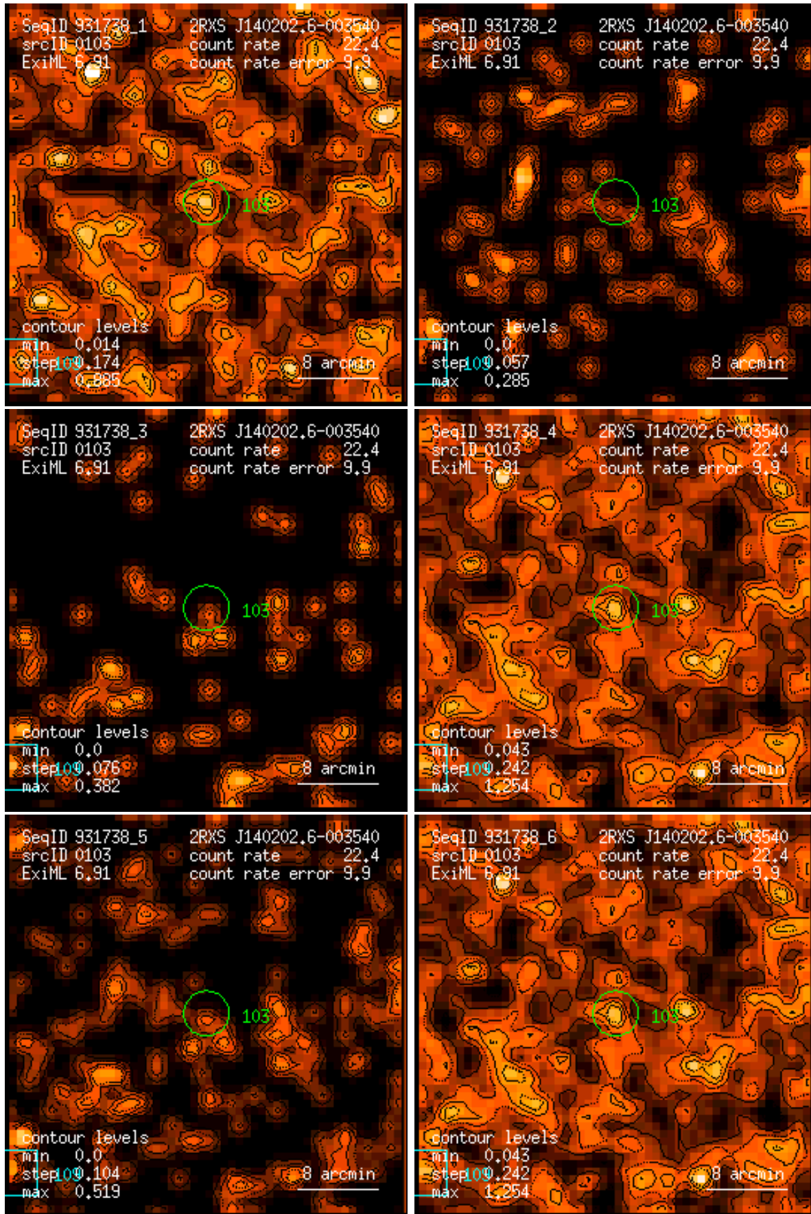
Figure 103: RASS 931738: detection 0103: band rate images, Gaussian filter: (1) PSPC channels 11 – 41, (2) 52 – 90, (3) 91 – 201, (4) 11 – 235, (5) 52 – 201, (6) 11 – 201. Broad band rates in counts/ks. Band rate contour levels in counts/ks/arcmin 2 .
