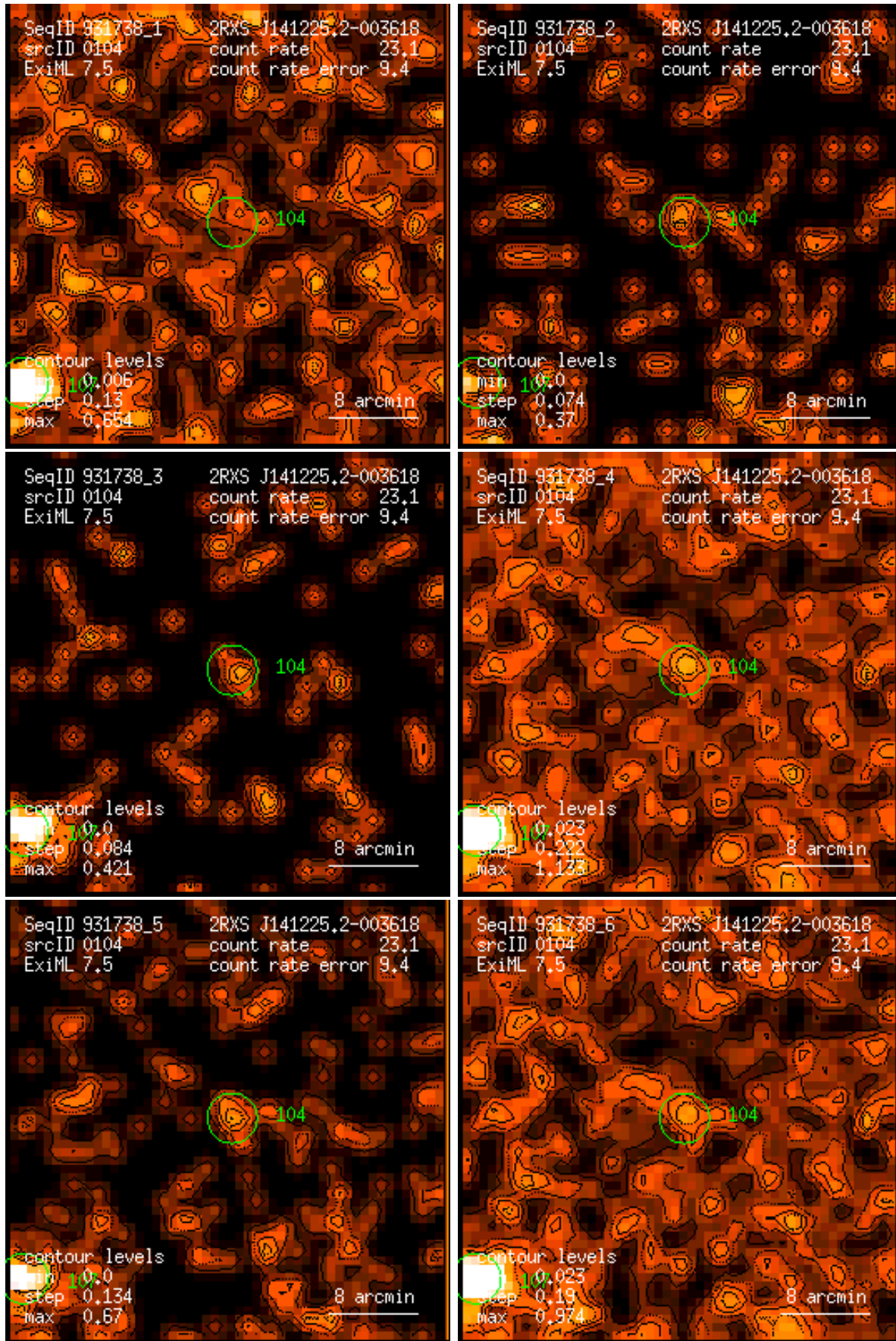
Figure 104: RASS 931738: detection 0104: band rate images, Gaussian filter: (1) PSPC channels 11 – 41, (2) 52 – 90, (3) 91 – 201, (4) 11 – 235, (5) 52 – 201, (6) 11 – 201. Broad band rates in counts/ks. Band rate contour levels in counts/ks/arcmin 2 .
