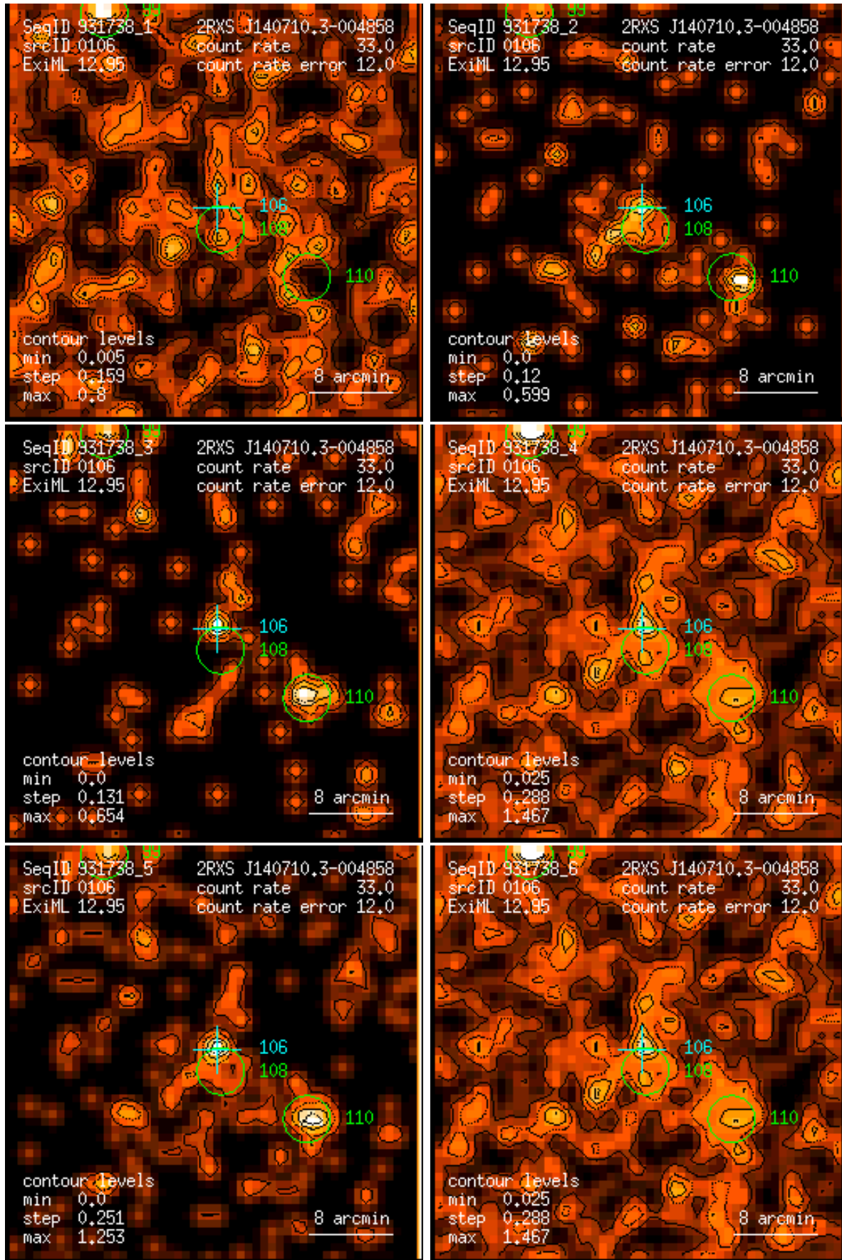
Figure 106: RASS 931738: detection 0106: band rate images, Gaussian filter: (1) PSPC channels 11 – 41, (2) 52 – 90, (3) 91 – 201, (4) 11 – 235, (5) 52 – 201, (6) 11 – 201. Broad band rates in counts/ks. Band rate contour levels in counts/ks/arcmin 2 .
