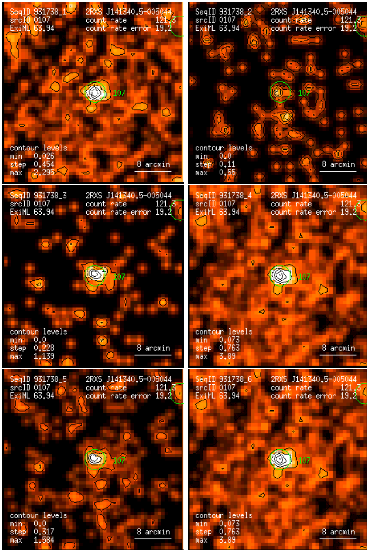
Figure 107: RASS 931738: detection 0107: band rate images, Gaussian filter: (1) PSPC channels 11 – 41, (2) 52 – 90, (3) 91 – 201, (4) 11 – 235, (5) 52 – 201, (6) 11 – 201. Broad band rates in counts/ks. Band rate contour levels in counts/ks/arcmin 2 .
