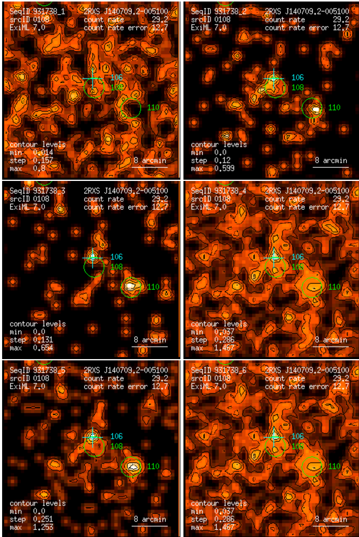
Figure 108: RASS 931738: detection 0108: band rate images, Gaussian filter: (1) PSPC channels 11 – 41, (2) 52 – 90, (3) 91 – 201, (4) 11 – 235, (5) 52 – 201, (6) 11 – 201. Broad band rates in counts/ks. Band rate contour levels in counts/ks/arcmin 2 .
