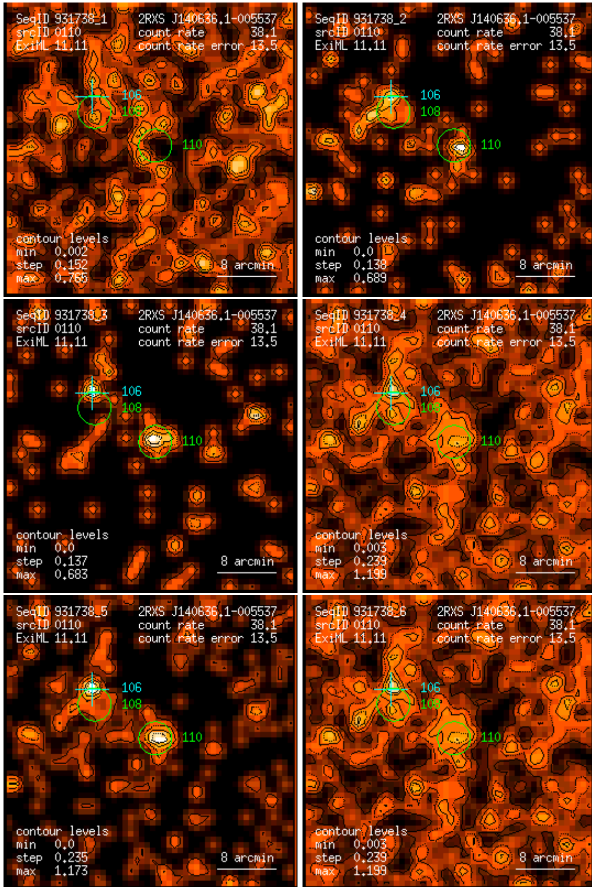
Figure 110: RASS 931738: detection 0110: band rate images, Gaussian filter: (1) PSPC channels 11 – 41, (2) 52 – 90, (3) 91 – 201, (4) 11 – 235, (5) 52 – 201, (6) 11 – 201. Broad band rates in counts/ks. Band rate contour levels in counts/ks/arcmin 2 .
