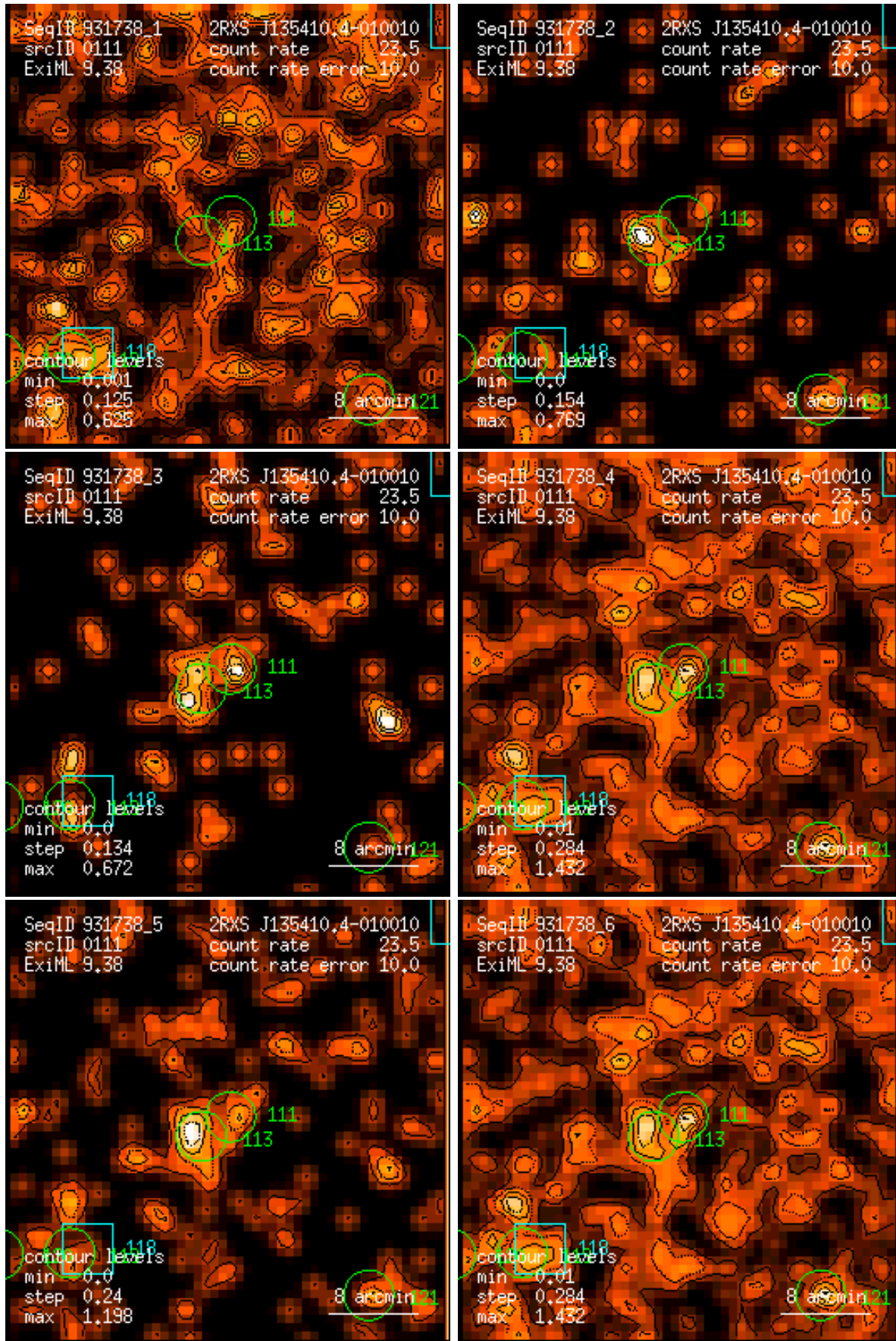
Figure 111: RASS 931738: detection 0111: band rate images, Gaussian filter: (1) PSPC channels 11 – 41, (2) 52 – 90, (3) 91 – 201, (4) 11 – 235, (5) 52 – 201, (6) 11 – 201. Broad band rates in counts/ks. Band rate contour levels in counts/ks/arcmin 2 .
