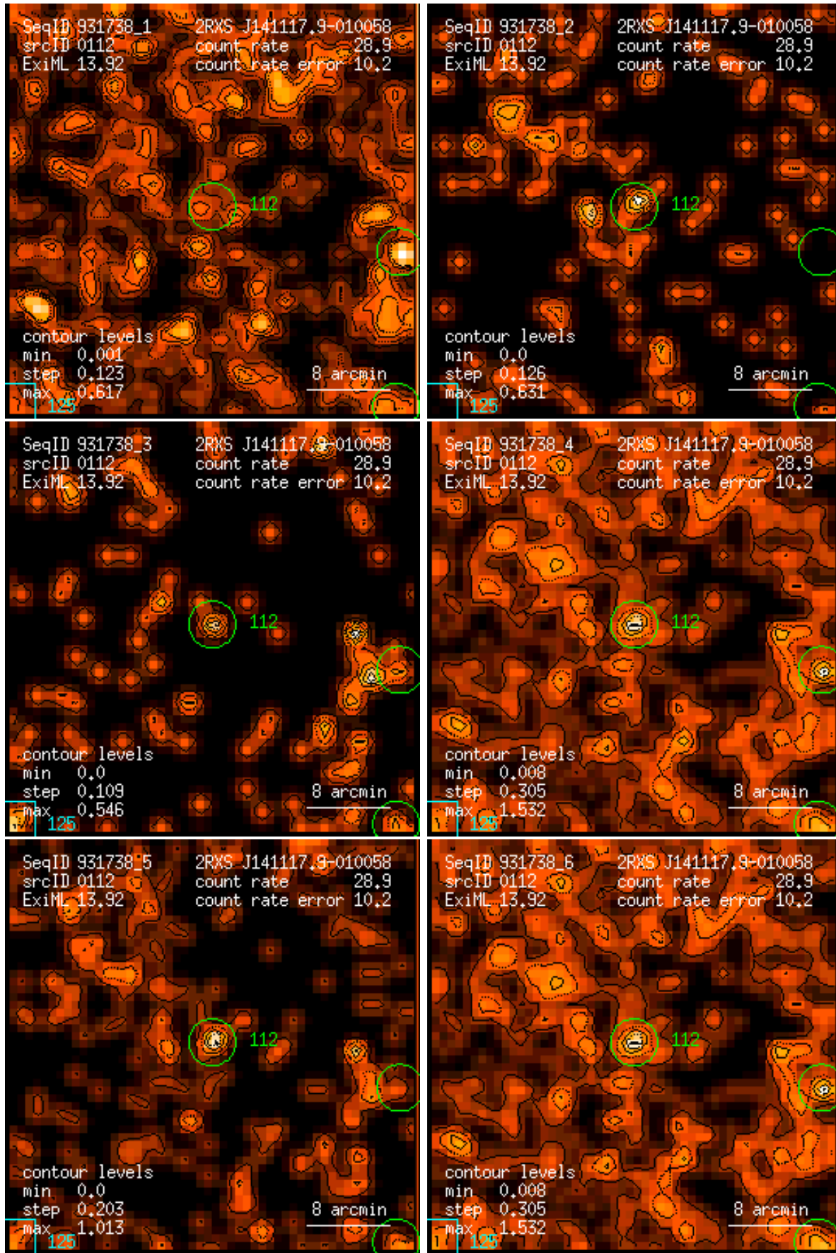
Figure 112: RASS 931738: detection 0112: band rate images, Gaussian filter: (1) PSPC channels 11 – 41, (2) 52 – 90, (3) 91 – 201, (4) 11 – 235, (5) 52 – 201, (6) 11 – 201. Broad band rates in counts/ks. Band rate contour levels in counts/ks/arcmin 2 .
