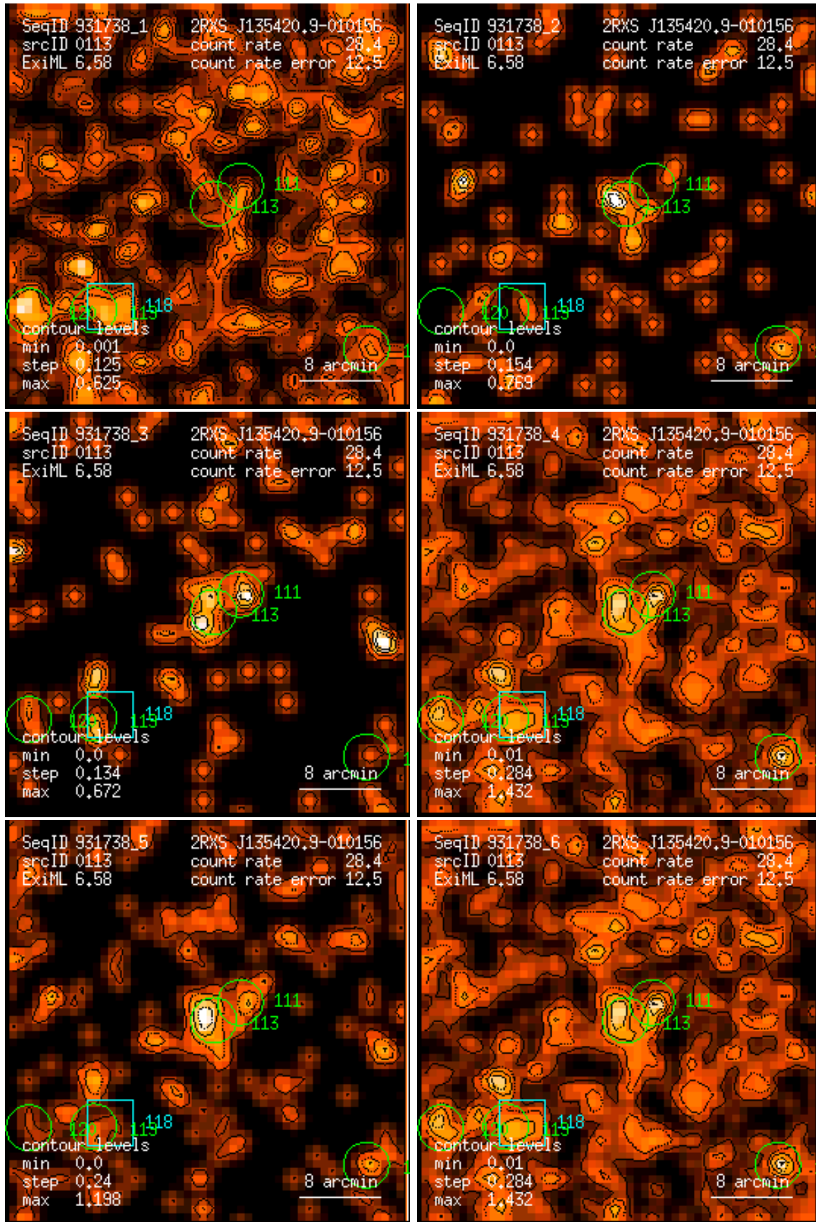
Figure 113: RASS 931738: detection 0113: band rate images, Gaussian filter: (1) PSPC channels 11 – 41, (2) 52 – 90, (3) 91 – 201, (4) 11 – 235, (5) 52 – 201, (6) 11 – 201. Broad band rates in counts/ks. Band rate contour levels in counts/ks/arcmin 2 .
