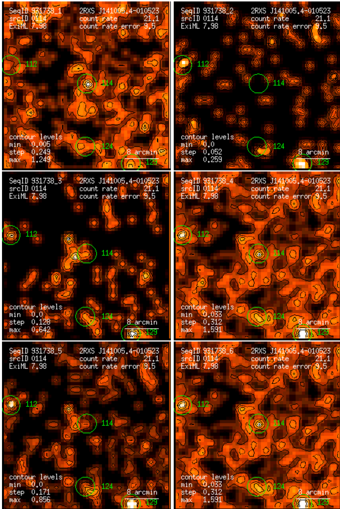
Figure 114: RASS 931738: detection 0114: band rate images, Gaussian filter: (1) PSPC channels 11 – 41, (2) 52 – 90, (3) 91 – 201, (4) 11 – 235, (5) 52 – 201, (6) 11 – 201. Broad band rates in counts/ks. Band rate contour levels in counts/ks/arcmin 2 .
