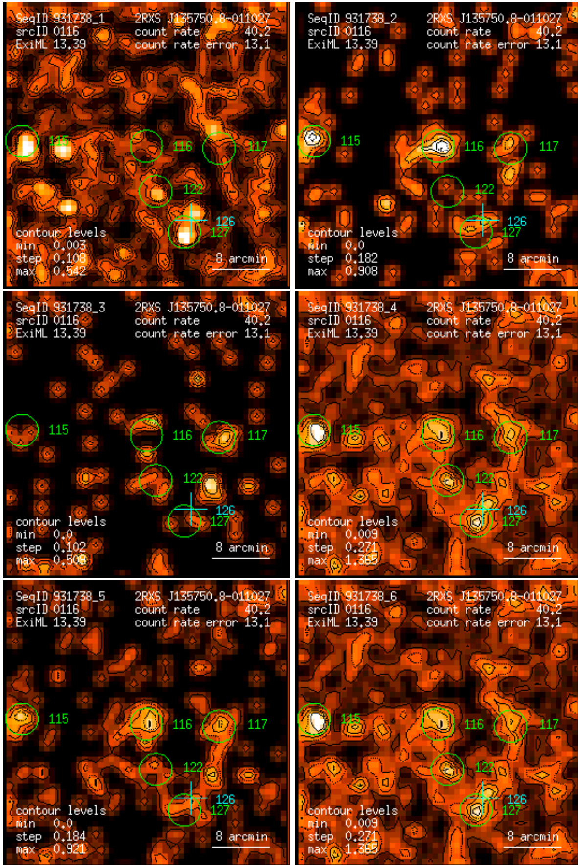
Figure 116: RASS 931738: detection 0116: band rate images, Gaussian filter: (1) PSPC channels 11 – 41, (2) 52 – 90, (3) 91 – 201, (4) 11 – 235, (5) 52 – 201, (6) 11 – 201. Broad band rates in counts/ks. Band rate contour levels in counts/ks/arcmin 2 .
