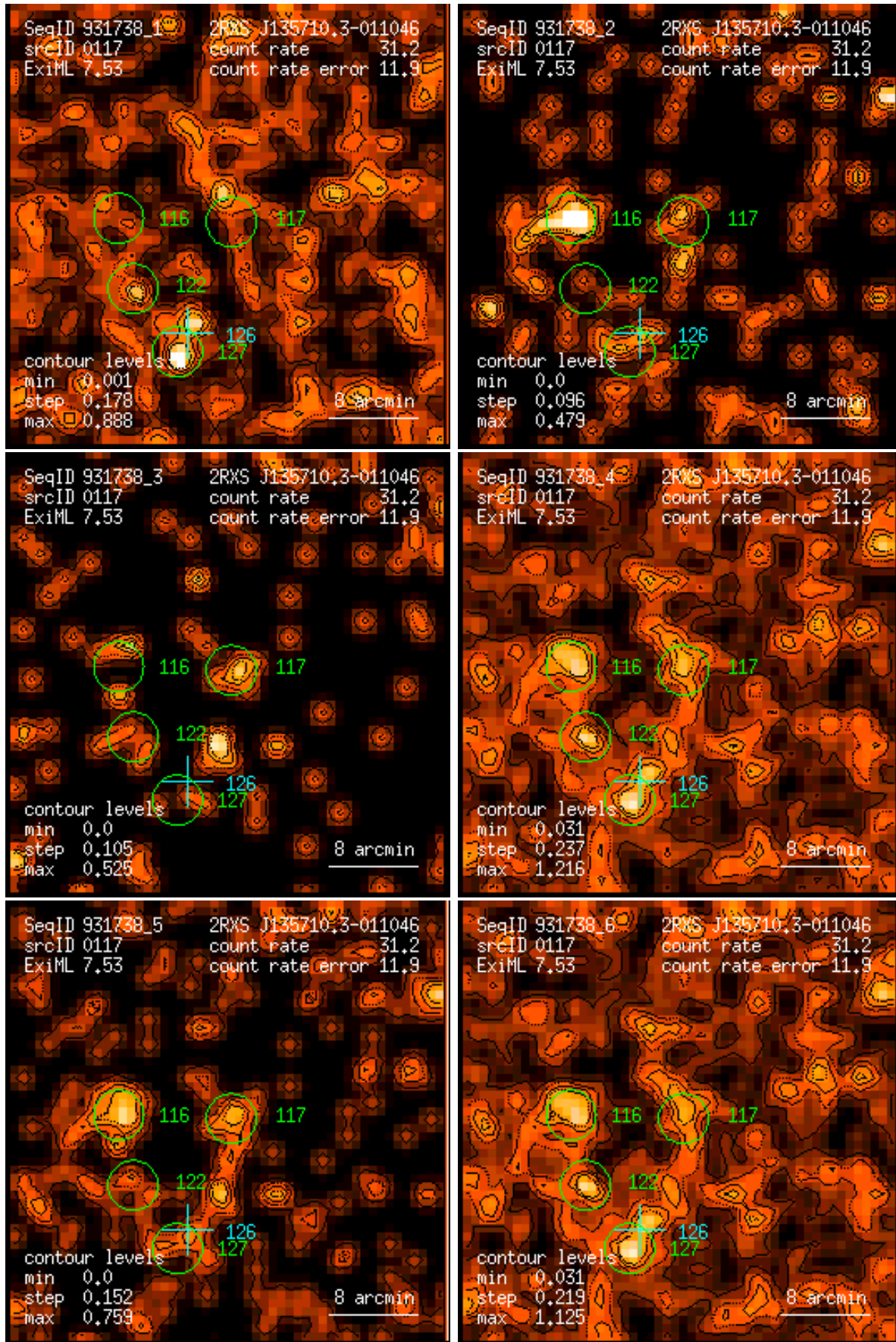
Figure 117: RASS 931738: detection 0117: band rate images, Gaussian filter: (1) PSPC channels 11 – 41, (2) 52 – 90, (3) 91 – 201, (4) 11 – 235, (5) 52 – 201, (6) 11 – 201. Broad band rates in counts/ks. Band rate contour levels in counts/ks/arcmin 2 .
