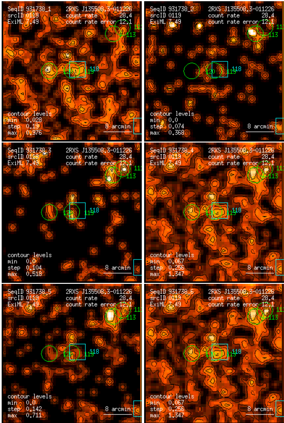
Figure 119: RASS 931738: detection 0119: band rate images, Gaussian filter: (1) PSPC channels 11 – 41, (2) 52 – 90, (3) 91 – 201, (4) 11 – 235, (5) 52 – 201, (6) 11 – 201. Broad band rates in counts/ks. Band rate contour levels in counts/ks/arcmin 2 .
