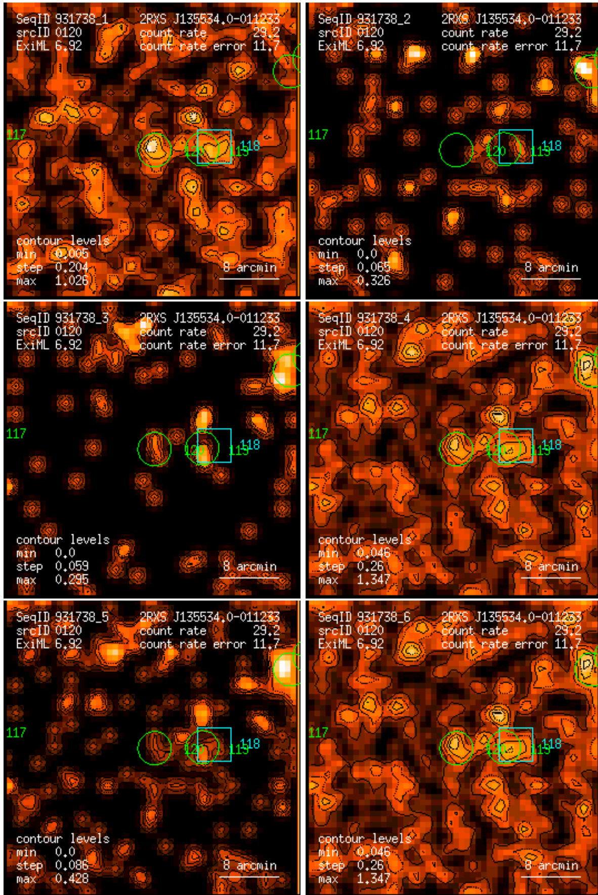
Figure 120: RASS 931738: detection 0120: band rate images, Gaussian filter: (1) PSPC channels 11 – 41, (2) 52 – 90, (3) 91 – 201, (4) 11 – 235, (5) 52 – 201, (6) 11 – 201. Broad band rates in counts/ks. Band rate contour levels in counts/ks/arcmin 2 .
