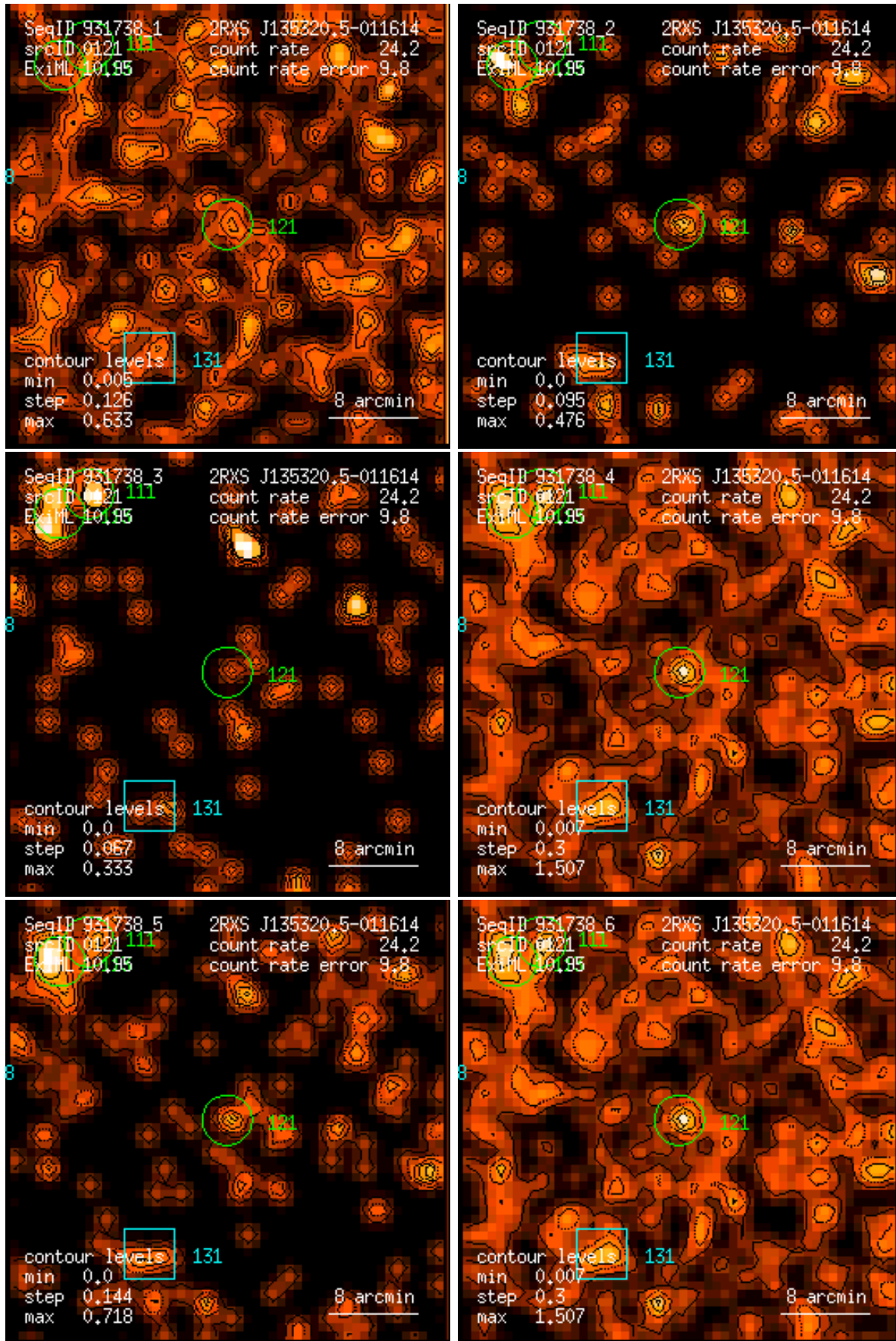
Figure 121: RASS 931738: detection 0121: band rate images, Gaussian filter: (1) PSPC channels 11 – 41, (2) 52 – 90, (3) 91 – 201, (4) 11 – 235, (5) 52 – 201, (6) 11 – 201. Broad band rates in counts/ks. Band rate contour levels in counts/ks/arcmin 2 .
