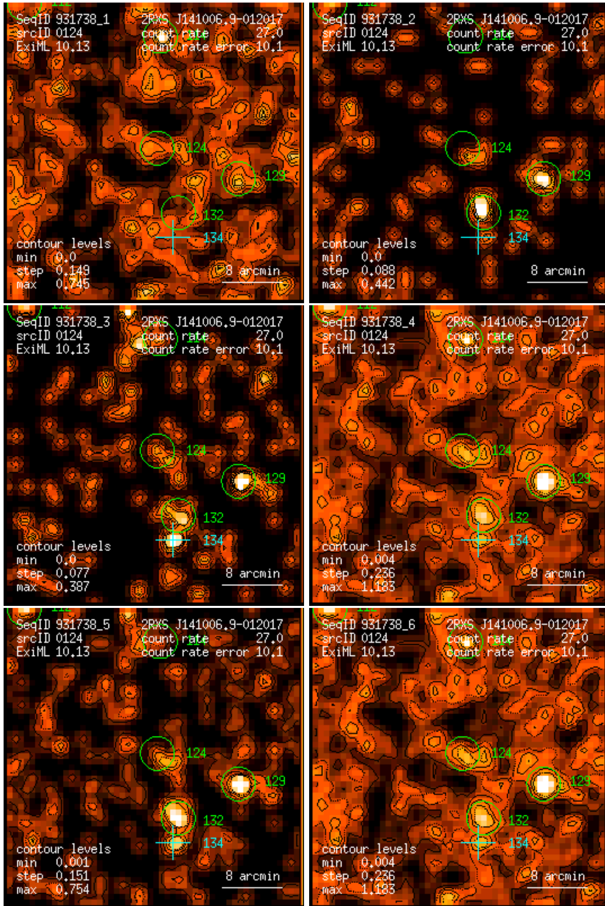
Figure 124: RASS 931738: detection 0124: band rate images, Gaussian filter: (1) PSPC channels 11 – 41, (2) 52 – 90, (3) 91 – 201, (4) 11 – 235, (5) 52 – 201, (6) 11 – 201. Broad band rates in counts/ks. Band rate contour levels in counts/ks/arcmin 2 .
