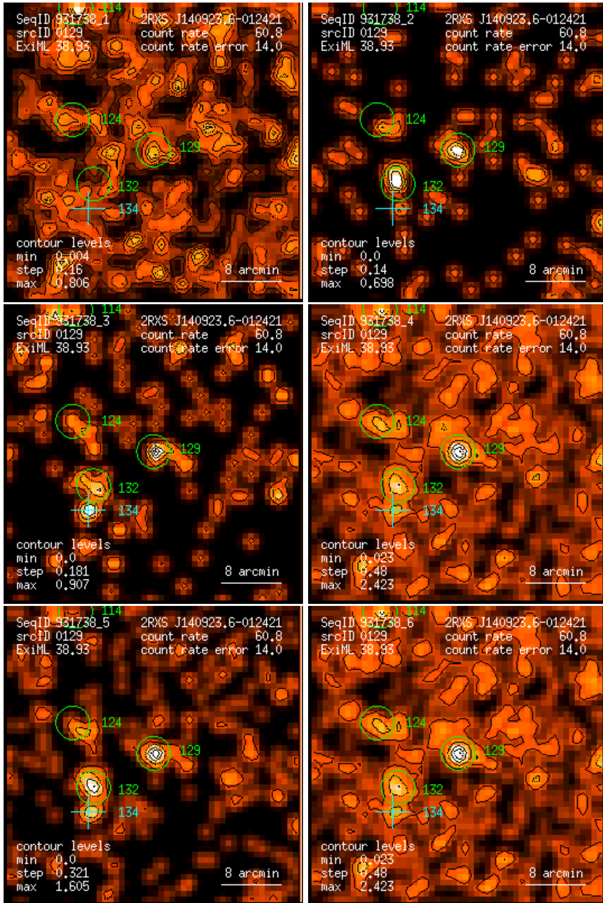
Figure 129: RASS 931738: detection 0129: band rate images, Gaussian filter: (1) PSPC channels 11 – 41, (2) 52 – 90, (3) 91 – 201, (4) 11 – 235, (5) 52 – 201, (6) 11 – 201. Broad band rates in counts/ks. Band rate contour levels in counts/ks/arcmin 2 .
