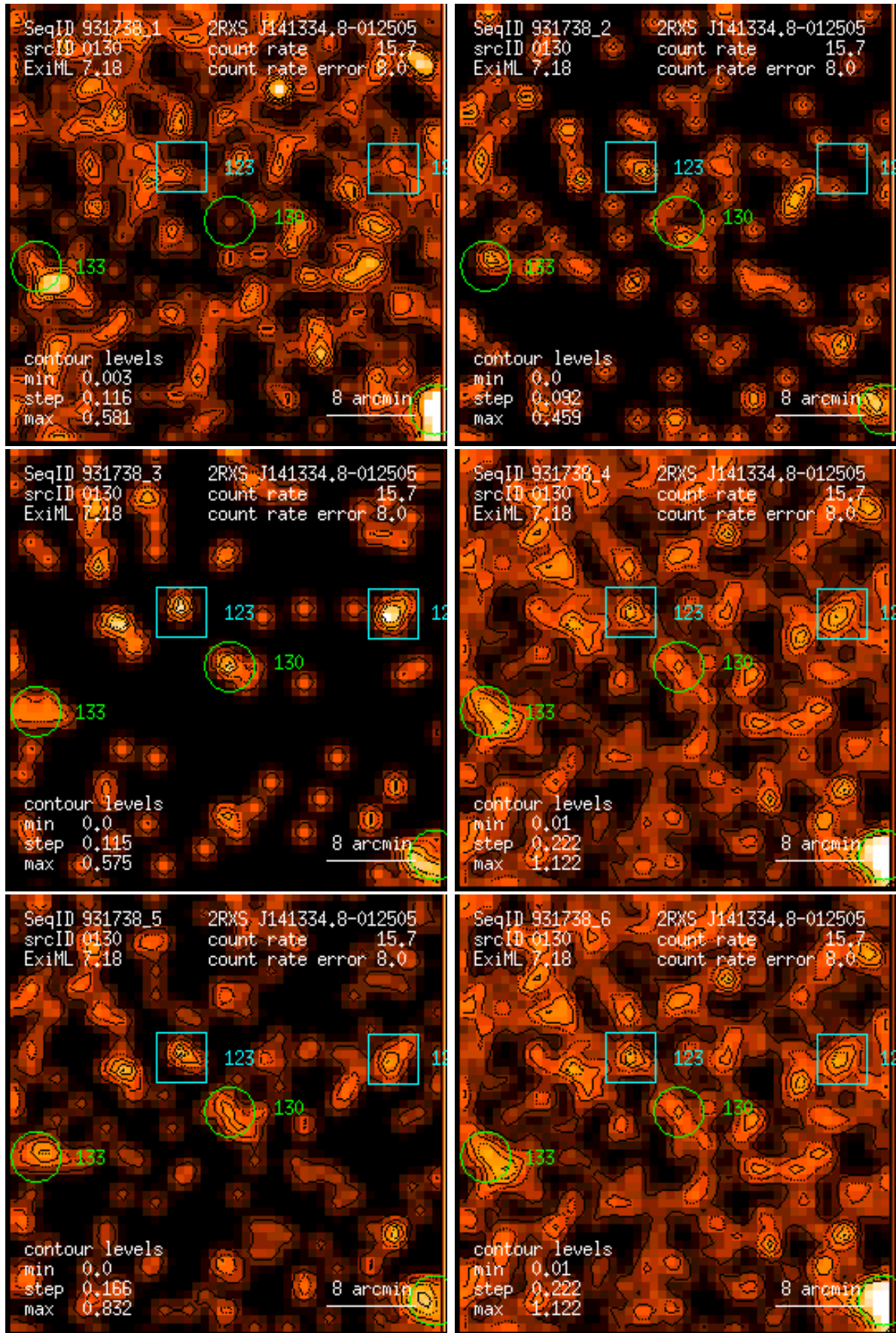
Figure 130: RASS 931738: detection 0130: band rate images, Gaussian filter: (1) PSPC channels 11 – 41, (2) 52 – 90, (3) 91 – 201, (4) 11 – 235, (5) 52 – 201, (6) 11 – 201. Broad band rates in counts/ks. Band rate contour levels in counts/ks/arcmin 2 .
