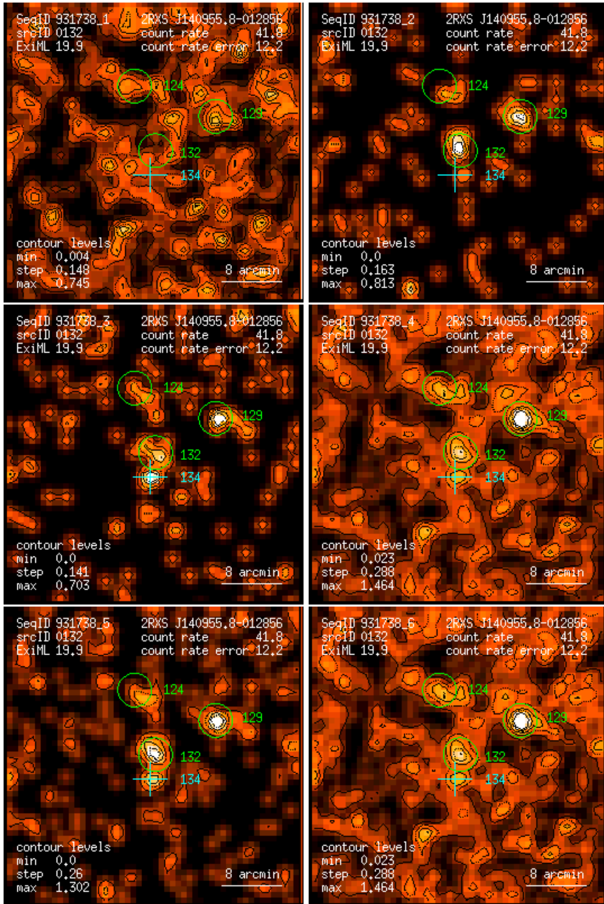
Figure 132: RASS 931738: detection 0132: band rate images, Gaussian filter: (1) PSPC channels 11 – 41, (2) 52 – 90, (3) 91 – 201, (4) 11 – 235, (5) 52 – 201, (6) 11 – 201. Broad band rates in counts/ks. Band rate contour levels in counts/ks/arcmin 2 .
