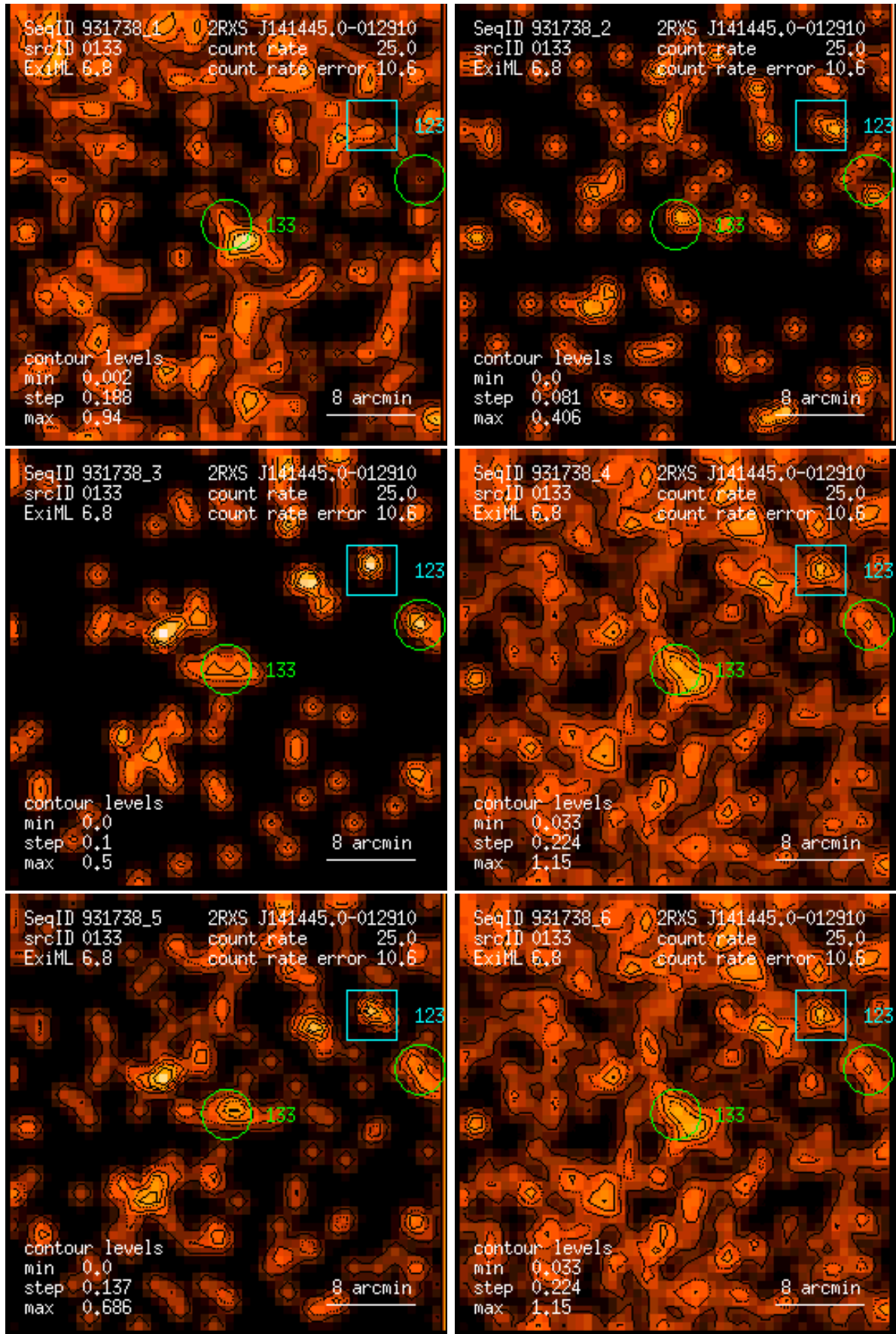
Figure 133: RASS 931738: detection 0133: band rate images, Gaussian filter: (1) PSPC channels 11 – 41, (2) 52 – 90, (3) 91 – 201, (4) 11 – 235, (5) 52 – 201, (6) 11 – 201. Broad band rates in counts/ks. Band rate contour levels in counts/ks/arcmin 2 .
