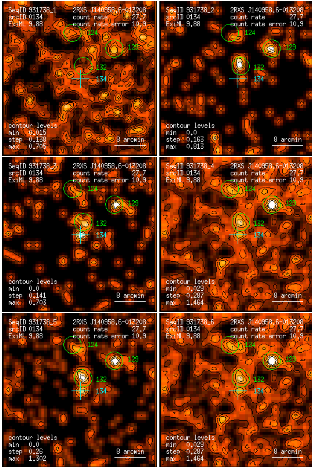
Figure 134: RASS 931738: detection 0134: band rate images, Gaussian filter: (1) PSPC channels 11 – 41, (2) 52 – 90, (3) 91 – 201, (4) 11 – 235, (5) 52 – 201, (6) 11 – 201. Broad band rates in counts/ks. Band rate contour levels in counts/ks/arcmin 2 .
