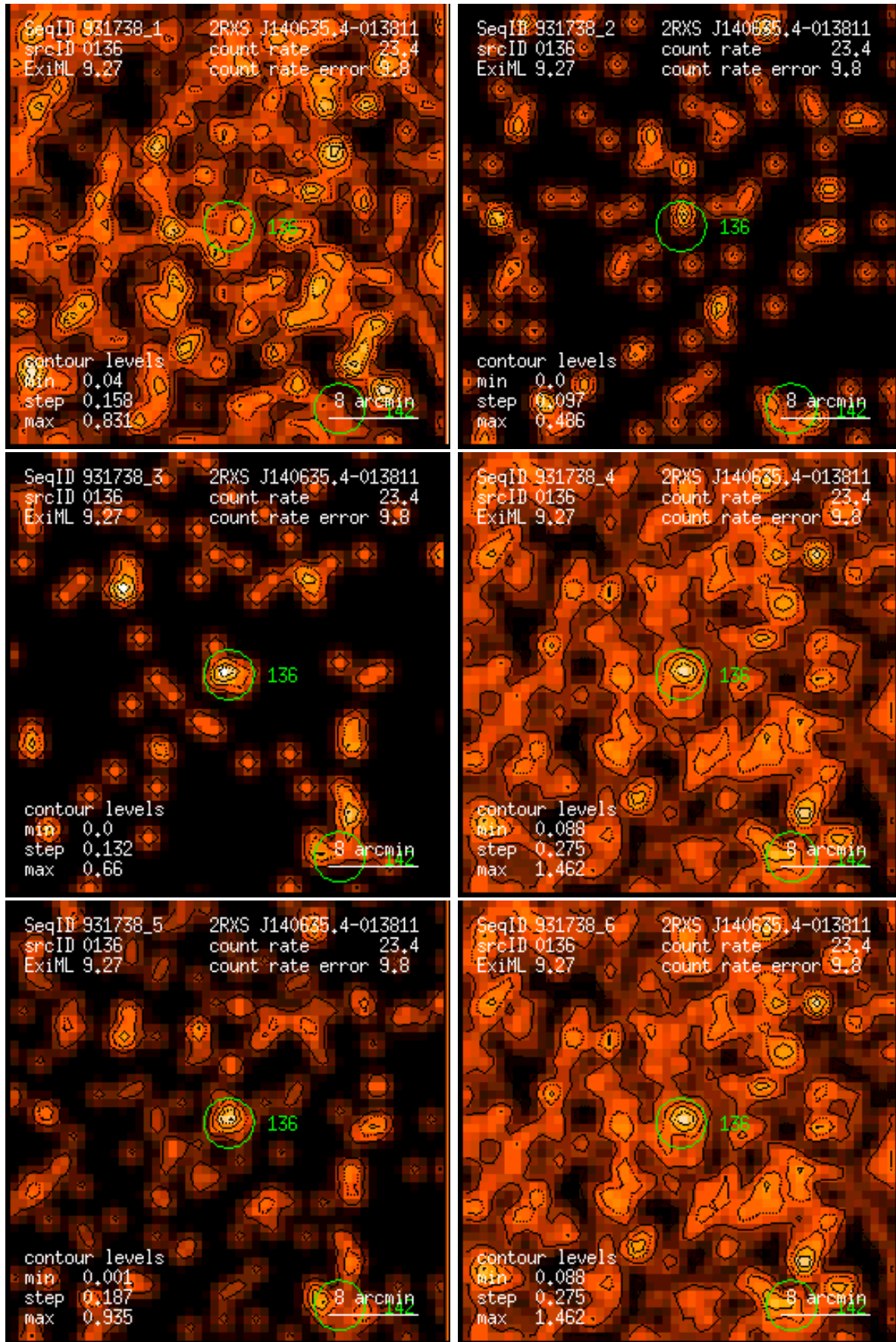
Figure 136: RASS 931738: detection 0136: band rate images, Gaussian filter: (1) PSPC channels 11 – 41, (2) 52 – 90, (3) 91 – 201, (4) 11 – 235, (5) 52 – 201, (6) 11 – 201. Broad band rates in counts/ks. Band rate contour levels in counts/ks/arcmin 2 .
