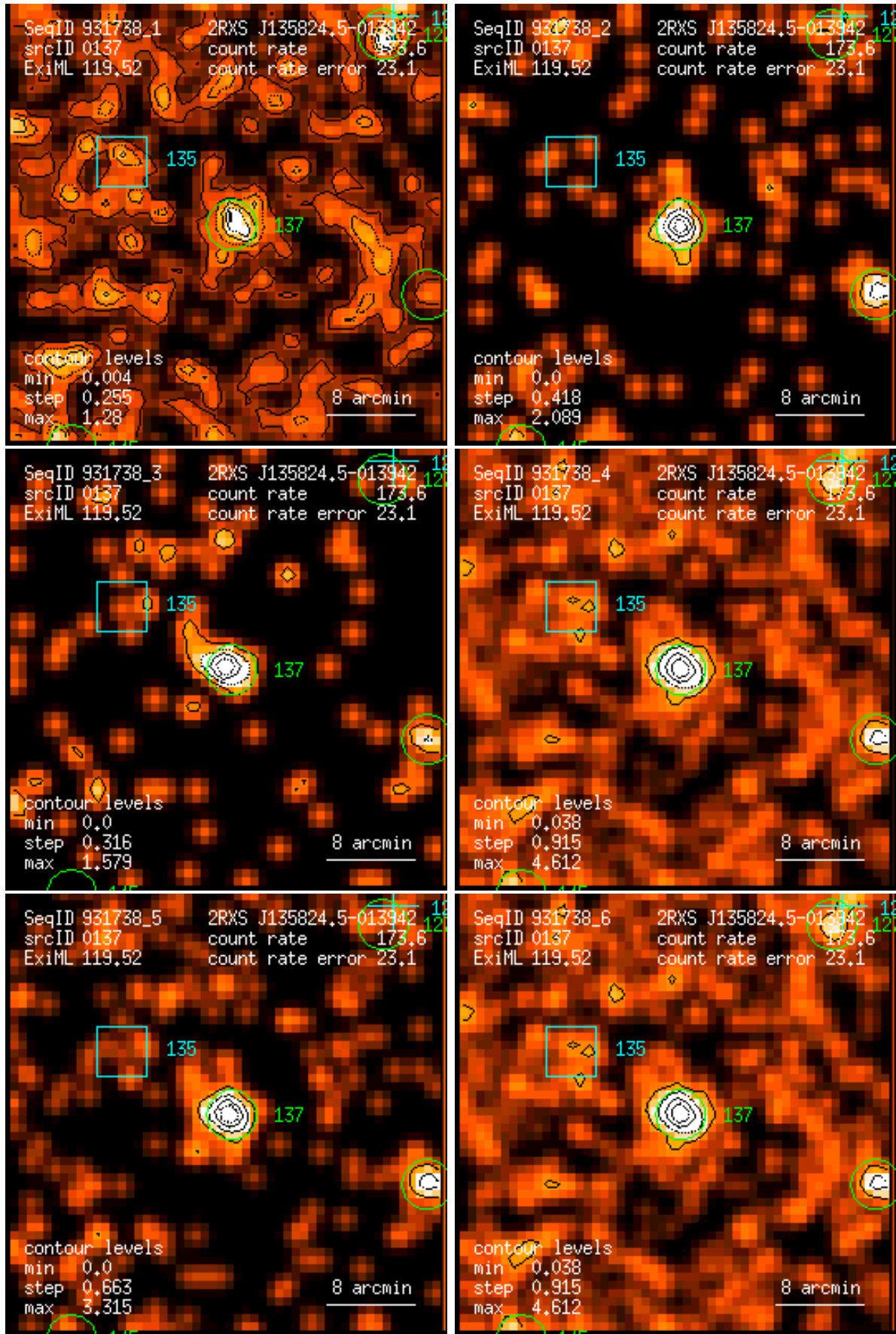
Figure 137: RASS 931738: detection 0137: band rate images, Gaussian filter: (1) PSPC channels 11 – 41, (2) 52 – 90, (3) 91 – 201, (4) 11 – 235, (5) 52 – 201, (6) 11 – 201. Broad band rates in counts/ks. Band rate contour levels in counts/ks/arcmin 2 .
