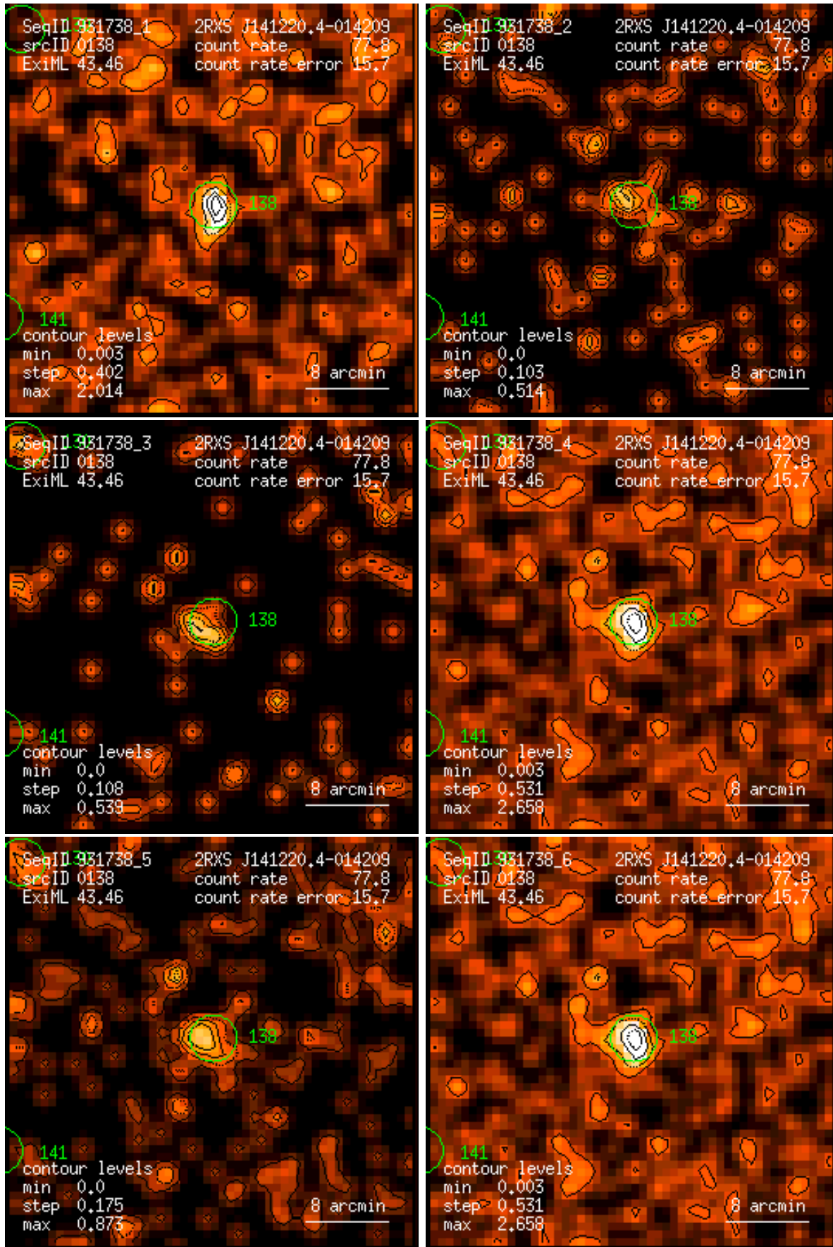
Figure 138: RASS 931738: detection 0138: band rate images, Gaussian filter: (1) PSPC channels 11 – 41, (2) 52 – 90, (3) 91 – 201, (4) 11 – 235, (5) 52 – 201, (6) 11 – 201. Broad band rates in counts/ks. Band rate contour levels in counts/ks/arcmin 2 .
