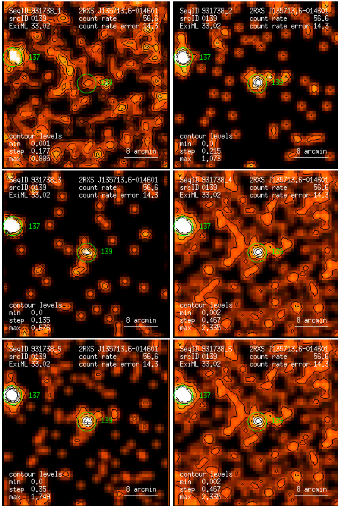
Figure 139: RASS 931738: detection 0139: band rate images, Gaussian filter: (1) PSPC channels 11 – 41, (2) 52 – 90, (3) 91 – 201, (4) 11 – 235, (5) 52 – 201, (6) 11 – 201. Broad band rates in counts/ks. Band rate contour levels in counts/ks/arcmin 2 .
