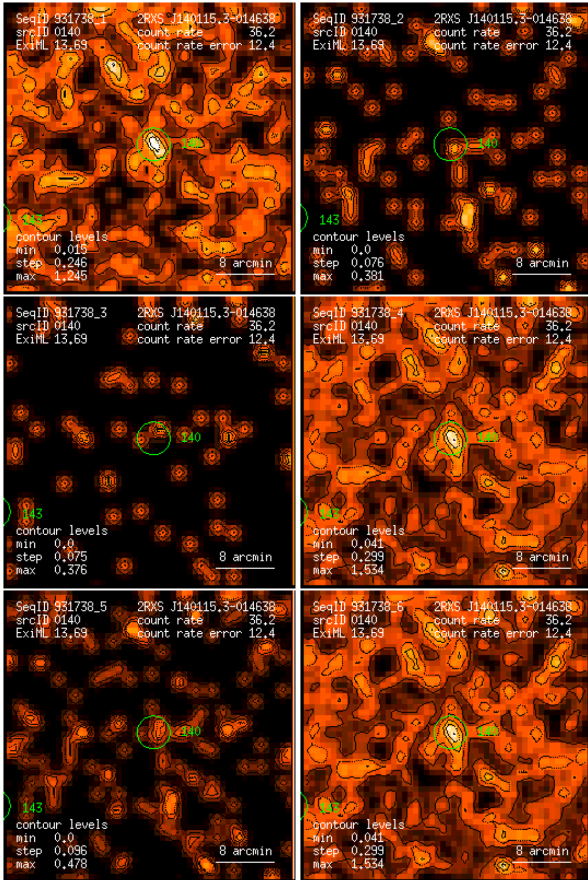
Figure 140: RASS 931738: detection 0140: band rate images, Gaussian filter: (1) PSPC channels 11 – 41, (2) 52 – 90, (3) 91 – 201, (4) 11 – 235, (5) 52 – 201, (6) 11 – 201. Broad band rates in counts/ks. Band rate contour levels in counts/ks/arcmin 2 .
