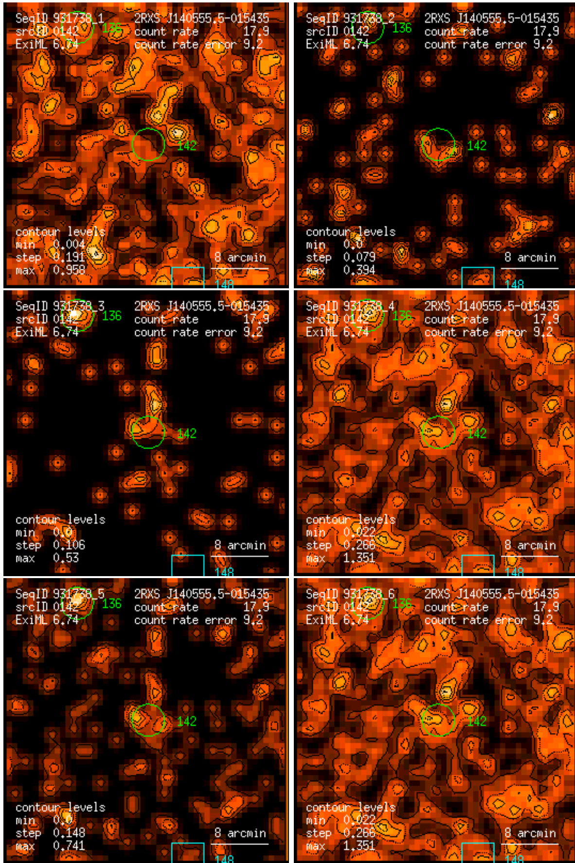
Figure 142: RASS 931738: detection 0142: band rate images, Gaussian filter: (1) PSPC channels 11 – 41, (2) 52 – 90, (3) 91 – 201, (4) 11 – 235, (5) 52 – 201, (6) 11 – 201. Broad band rates in counts/ks. Band rate contour levels in counts/ks/arcmin 2 .
