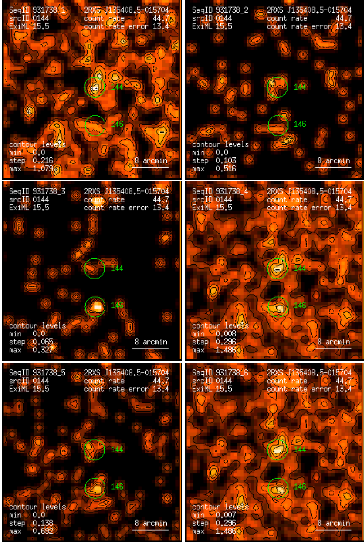
Figure 144: RASS 931738: detection 0144: band rate images, Gaussian filter: (1) PSPC channels 11 – 41, (2) 52 – 90, (3) 91 – 201, (4) 11 – 235, (5) 52 – 201, (6) 11 – 201. Broad band rates in counts/ks. Band rate contour levels in counts/ks/arcmin 2 .
