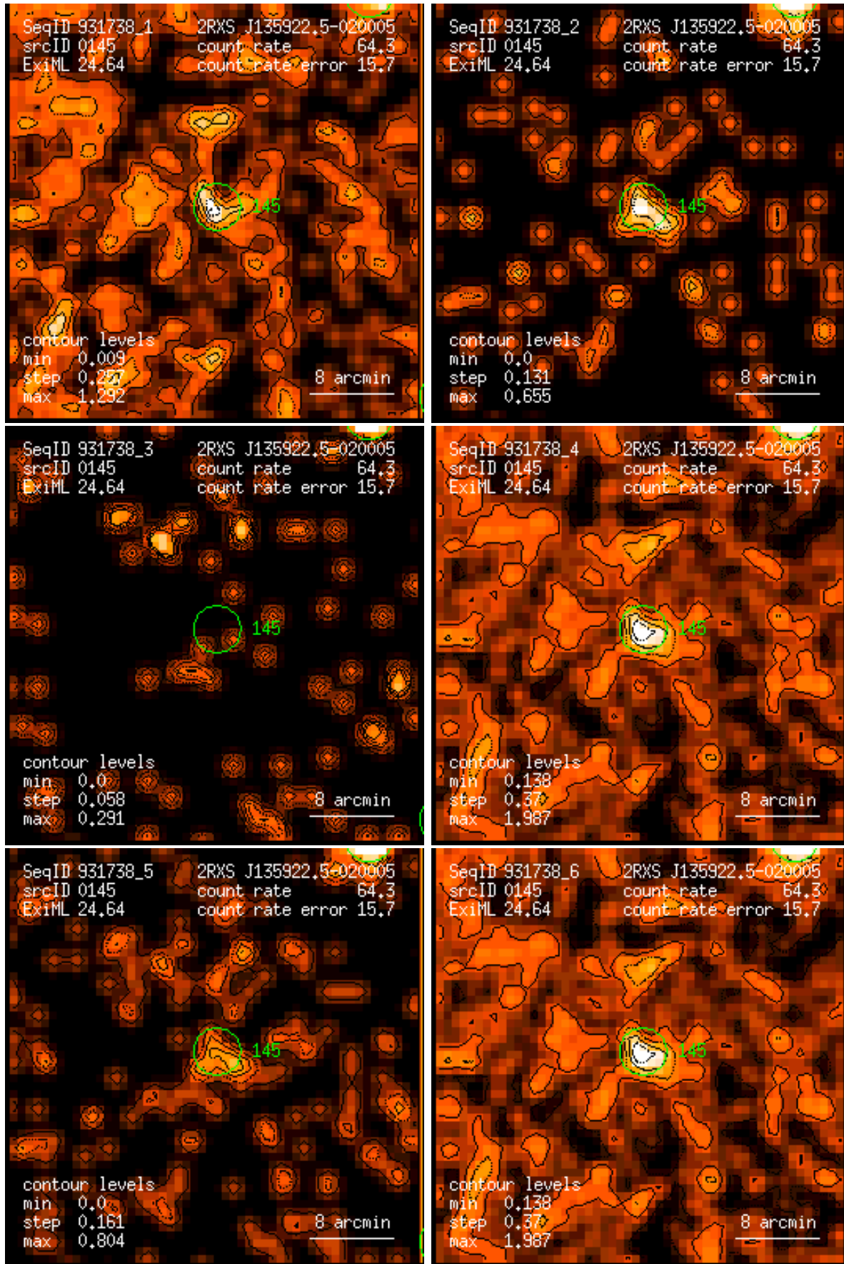
Figure 145: RASS 931738: detection 0145: band rate images, Gaussian filter: (1) PSPC channels 11 – 41, (2) 52 – 90, (3) 91 – 201, (4) 11 – 235, (5) 52 – 201, (6) 11 – 201. Broad band rates in counts/ks. Band rate contour levels in counts/ks/arcmin 2 .
