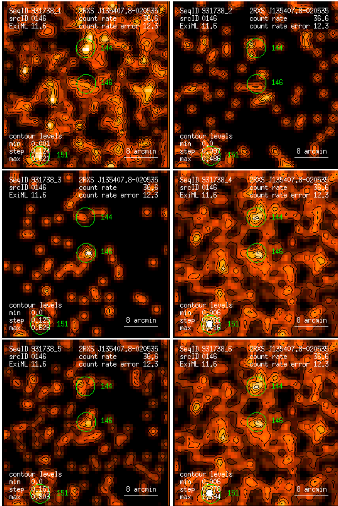
Figure 146: RASS 931738: detection 0146: band rate images, Gaussian filter: (1) PSPC channels 11 – 41, (2) 52 – 90, (3) 91 – 201, (4) 11 – 235, (5) 52 – 201, (6) 11 – 201. Broad band rates in counts/ks. Band rate contour levels in counts/ks/arcmin 2 .
