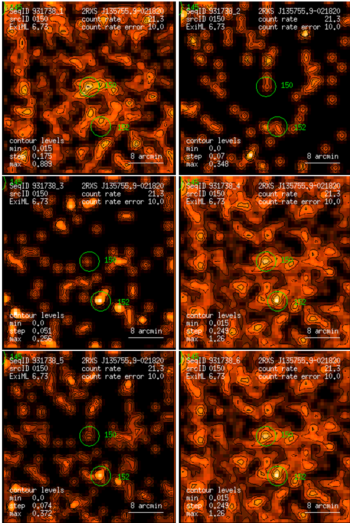
Figure 150: RASS 931738: detection 0150: band rate images, Gaussian filter: (1) PSPC channels 11 – 41, (2) 52 – 90, (3) 91 – 201, (4) 11 – 235, (5) 52 – 201, (6) 11 – 201. Broad band rates in counts/ks. Band rate contour levels in counts/ks/arcmin 2 .
