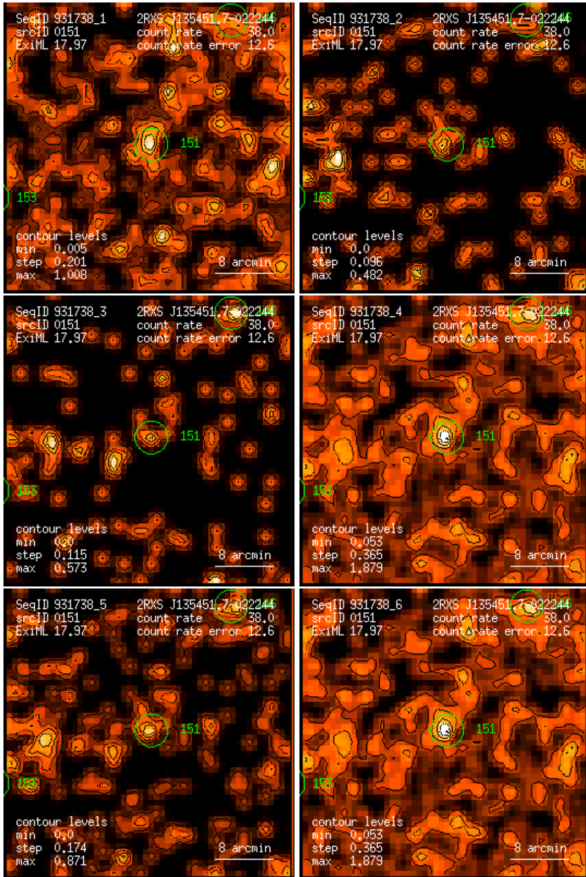
Figure 151: RASS 931738: detection 0151: band rate images, Gaussian filter: (1) PSPC channels 11 – 41, (2) 52 – 90, (3) 91 – 201, (4) 11 – 235, (5) 52 – 201, (6) 11 – 201. Broad band rates in counts/ks. Band rate contour levels in counts/ks/arcmin 2 .
