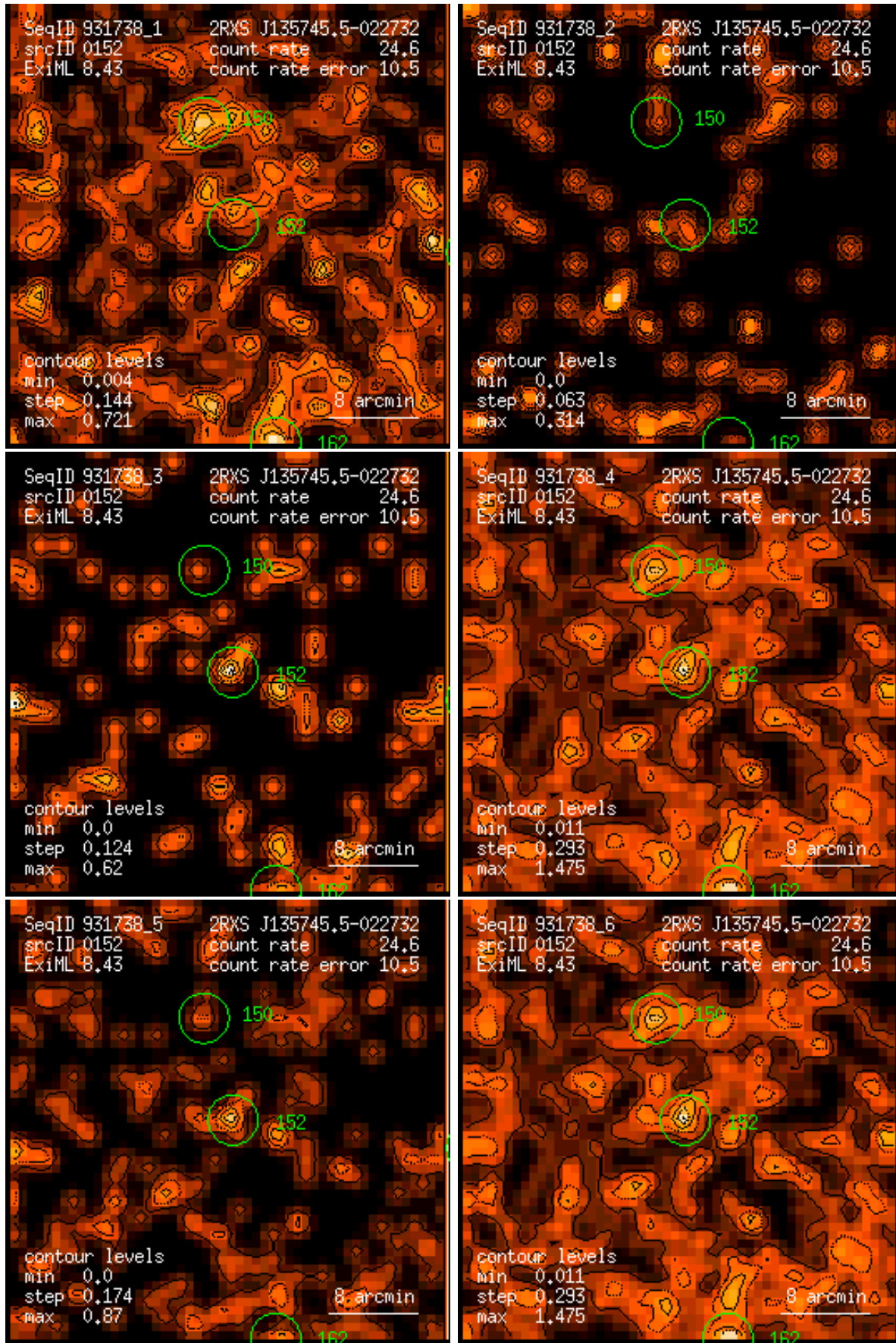
Figure 152: RASS 931738: detection 0152: band rate images, Gaussian filter: (1) PSPC channels 11 – 41, (2) 52 – 90, (3) 91 – 201, (4) 11 – 235, (5) 52 – 201, (6) 11 – 201. Broad band rates in counts/ks. Band rate contour levels in counts/ks/arcmin 2 .
