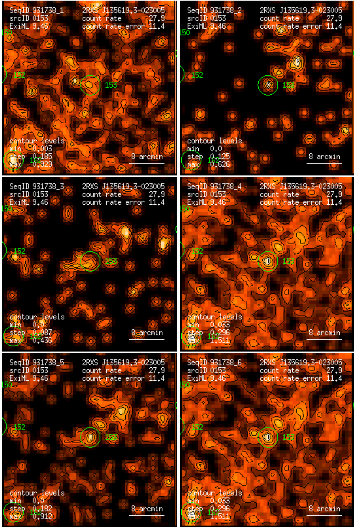
Figure 153: RASS 931738: detection 0153: band rate images, Gaussian filter: (1) PSPC channels 11 – 41, (2) 52 – 90, (3) 91 – 201, (4) 11 – 235, (5) 52 – 201, (6) 11 – 201. Broad band rates in counts/ks. Band rate contour levels in counts/ks/arcmin 2 .
