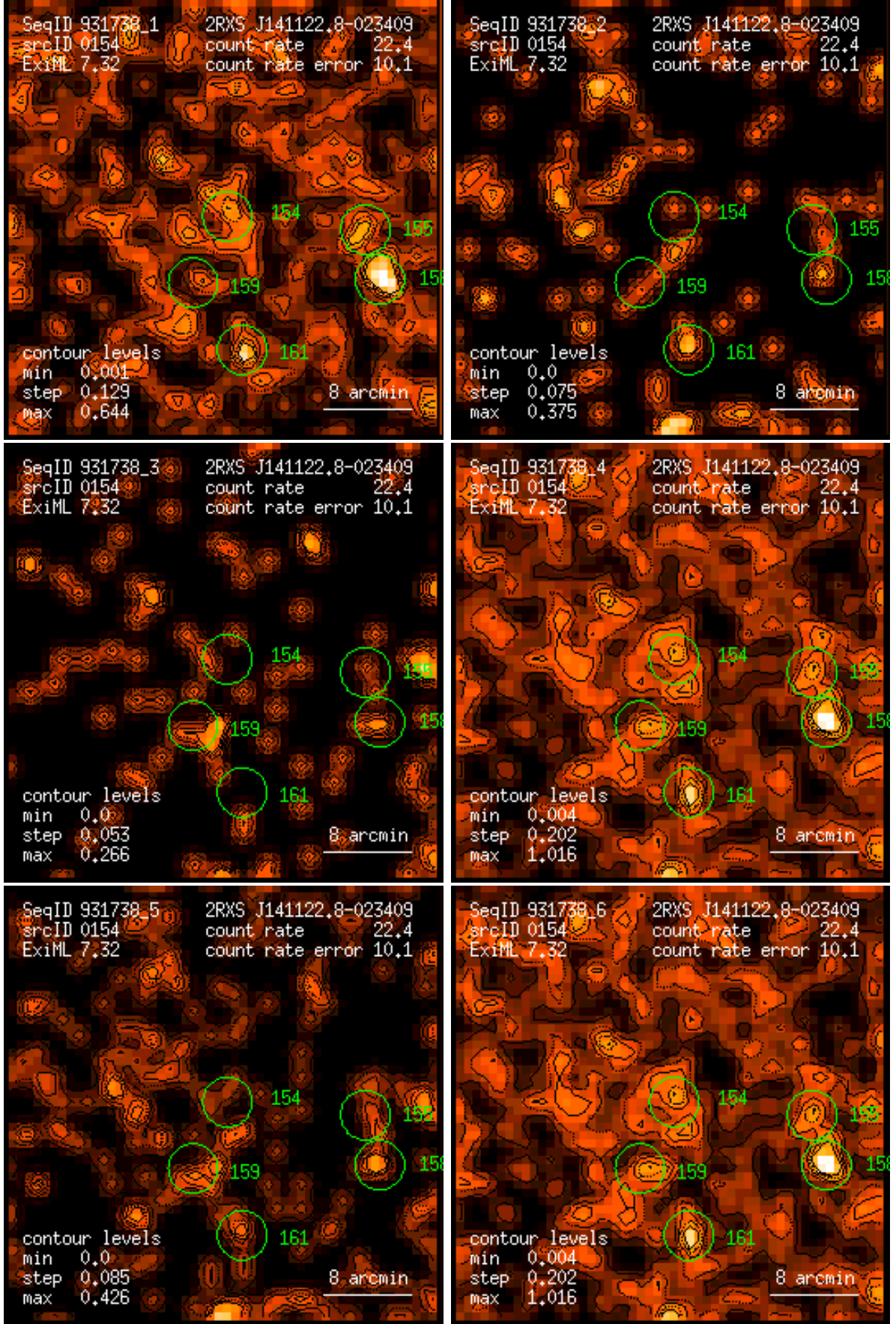
Figure 154: RASS 931738: detection 0154: band rate images, Gaussian filter: (1) PSPC channels 11 – 41, (2) 52 – 90, (3) 91 – 201, (4) 11 – 235, (5) 52 – 201, (6) 11 – 201. Broad band rates in counts/ks. Band rate contour levels in counts/ks/arcmin 2 .
