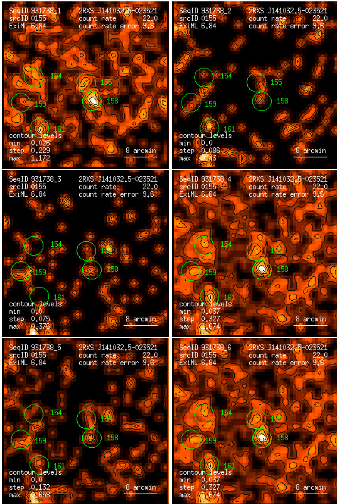
Figure 155: RASS 931738: detection 0155: band rate images, Gaussian filter: (1) PSPC channels 11 – 41, (2) 52 – 90, (3) 91 – 201, (4) 11 – 235, (5) 52 – 201, (6) 11 – 201. Broad band rates in counts/ks. Band rate contour levels in counts/ks/arcmin 2 .
