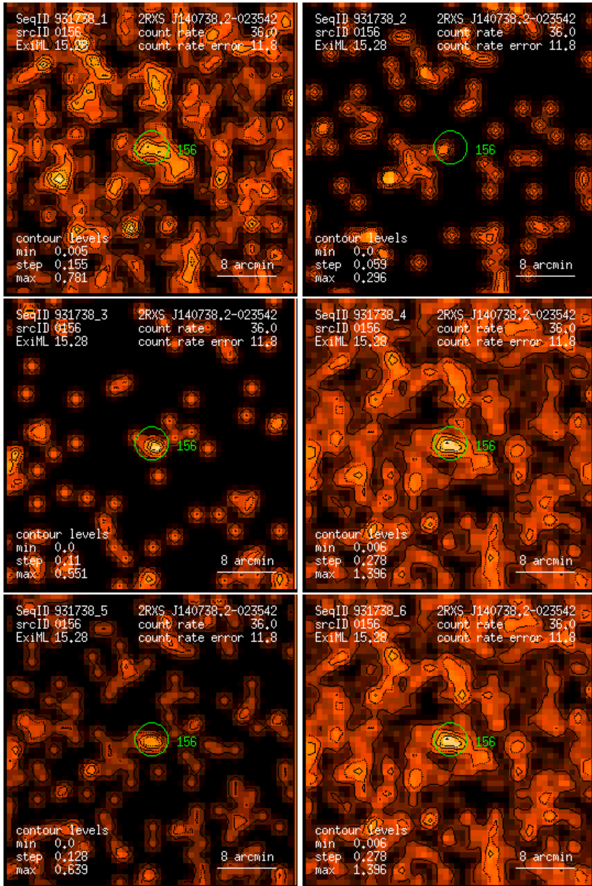
Figure 156: RASS 931738: detection 0156: band rate images, Gaussian filter: (1) PSPC channels 11 – 41, (2) 52 – 90, (3) 91 – 201, (4) 11 – 235, (5) 52 – 201, (6) 11 – 201. Broad band rates in counts/ks. Band rate contour levels in counts/ks/arcmin 2 .
