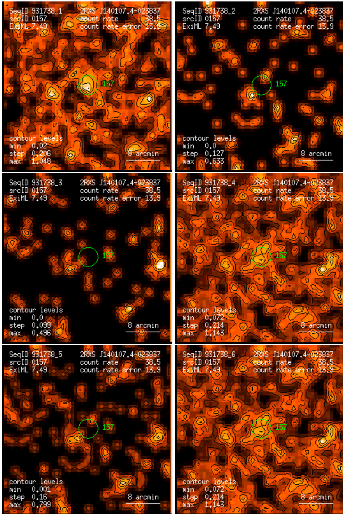
Figure 157: RASS 931738: detection 0157: band rate images, Gaussian filter: (1) PSPC channels 11 – 41, (2) 52 – 90, (3) 91 – 201, (4) 11 – 235, (5) 52 – 201, (6) 11 – 201. Broad band rates in counts/ks. Band rate contour levels in counts/ks/arcmin 2 .
