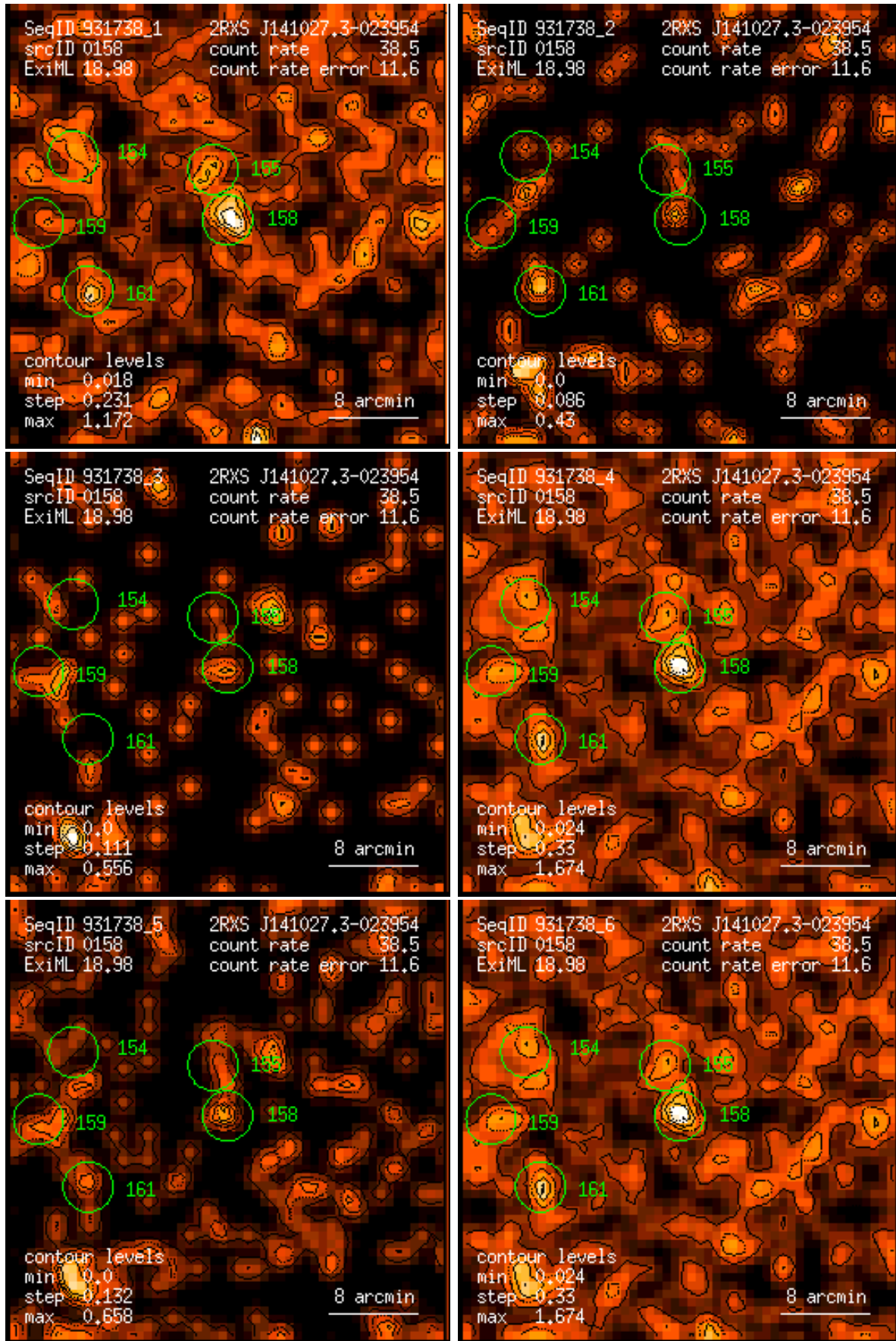
Figure 158: RASS 931738: detection 0158: band rate images, Gaussian filter: (1) PSPC channels 11 – 41, (2) 52 – 90, (3) 91 – 201, (4) 11 – 235, (5) 52 – 201, (6) 11 – 201. Broad band rates in counts/ks. Band rate contour levels in counts/ks/arcmin 2 .
