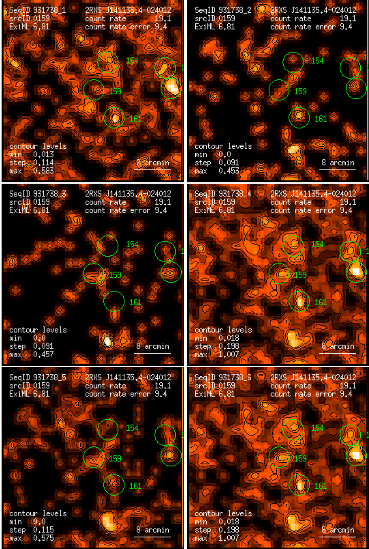
Figure 159: RASS 931738: detection 0159: band rate images, Gaussian filter: (1) PSPC channels 11 – 41, (2) 52 – 90, (3) 91 – 201, (4) 11 – 235, (5) 52 – 201, (6) 11 – 201. Broad band rates in counts/ks. Band rate contour levels in counts/ks/arcmin 2 .
