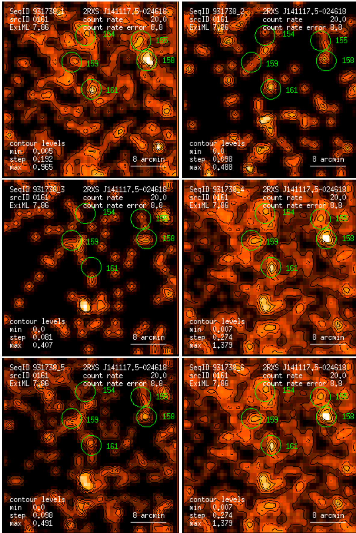
Figure 161: RASS 931738: detection 0161: band rate images, Gaussian filter: (1) PSPC channels 11 – 41, (2) 52 – 90, (3) 91 – 201, (4) 11 – 235, (5) 52 – 201, (6) 11 – 201. Broad band rates in counts/ks. Band rate contour levels in counts/ks/arcmin 2 .
