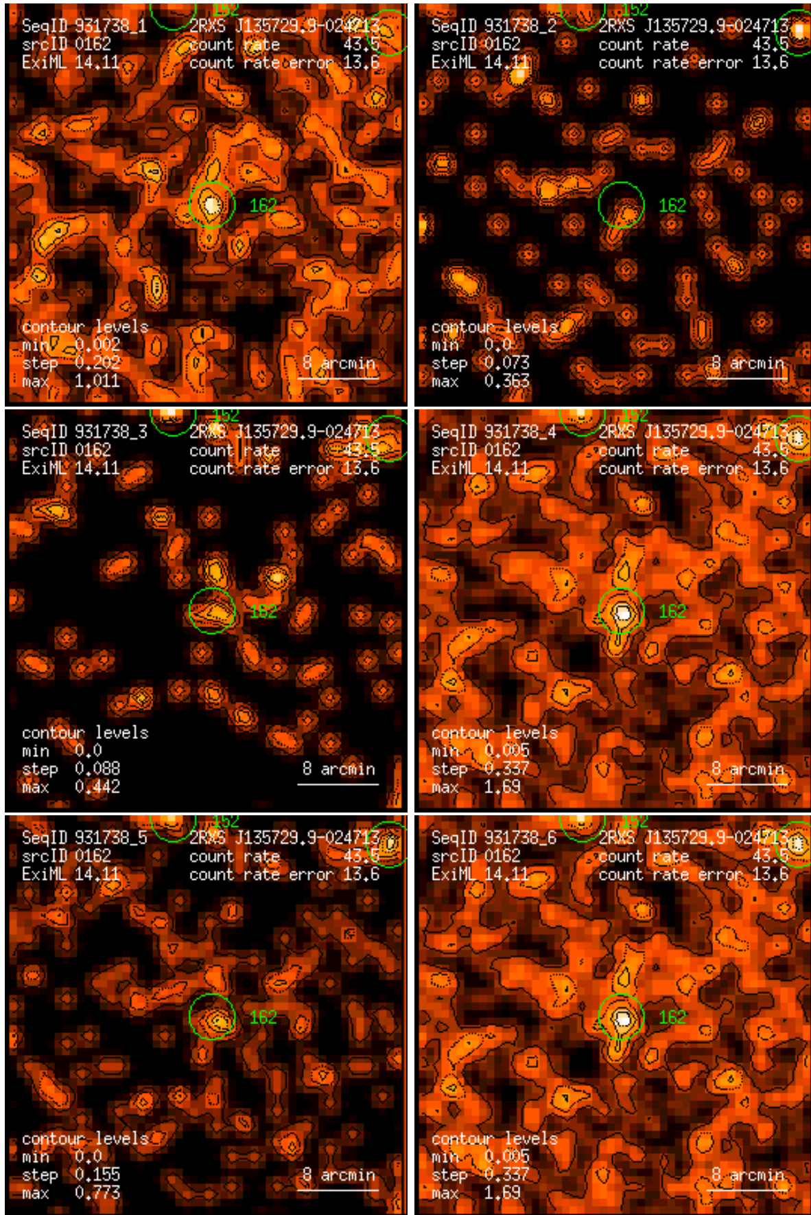
Figure 162: RASS 931738: detection 0162: band rate images, Gaussian filter: (1) PSPC channels 11 – 41, (2) 52 – 90, (3) 91 – 201, (4) 11 – 235, (5) 52 – 201, (6) 11 – 201. Broad band rates in counts/ks. Band rate contour levels in counts/ks/arcmin 2 .
