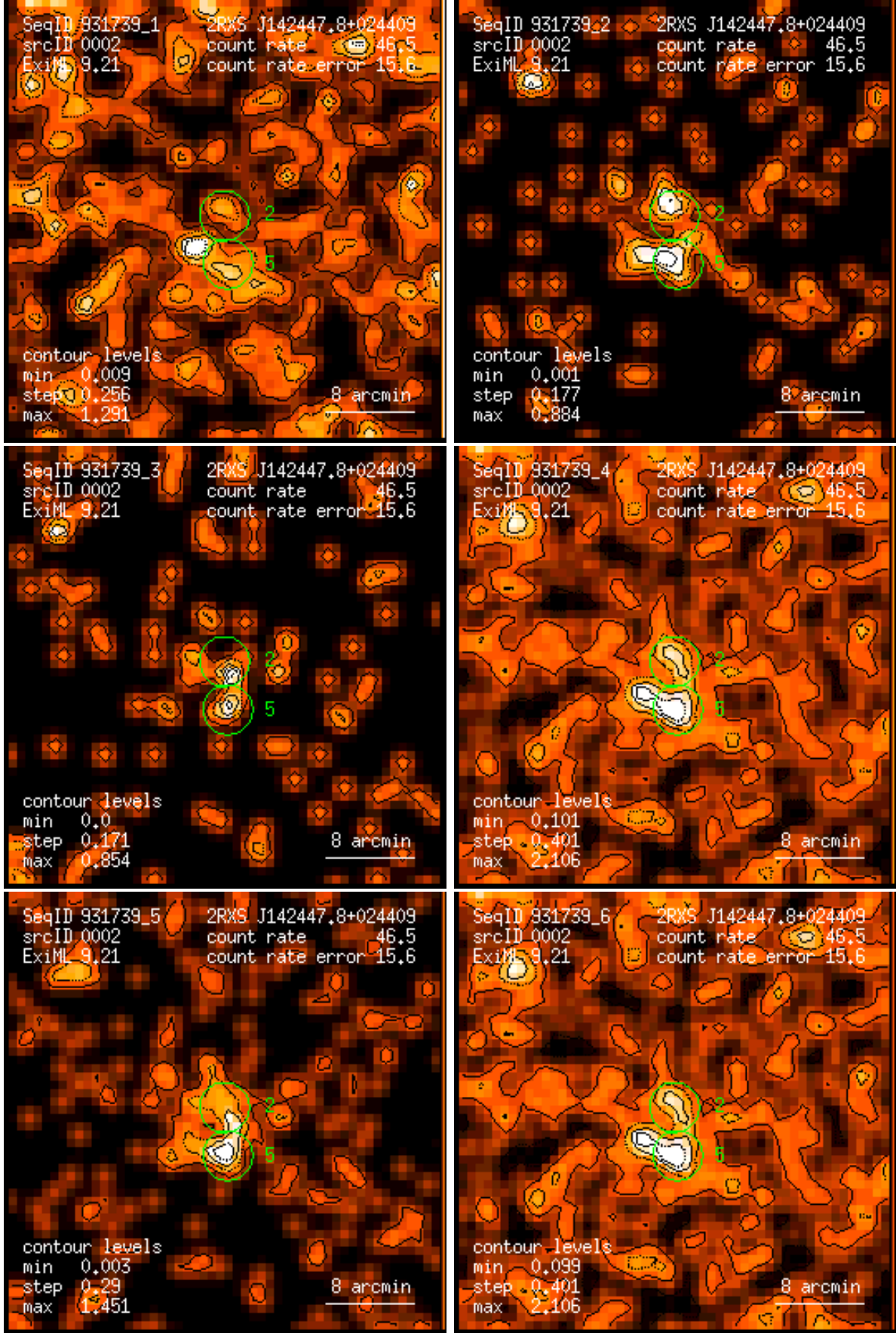
Figure 2: RASS 931739: detection 0002: band rate images, Gaussian filter: (1) PSPC channels 11 – 41, (2) 52 – 90, (3) 91 – 201, (4) 11 – 235, (5) 52 – 201, (6) 11 – 201. Broad band rates in counts/ks. Band rate contour levels in counts/ks/arcmin 2 .
