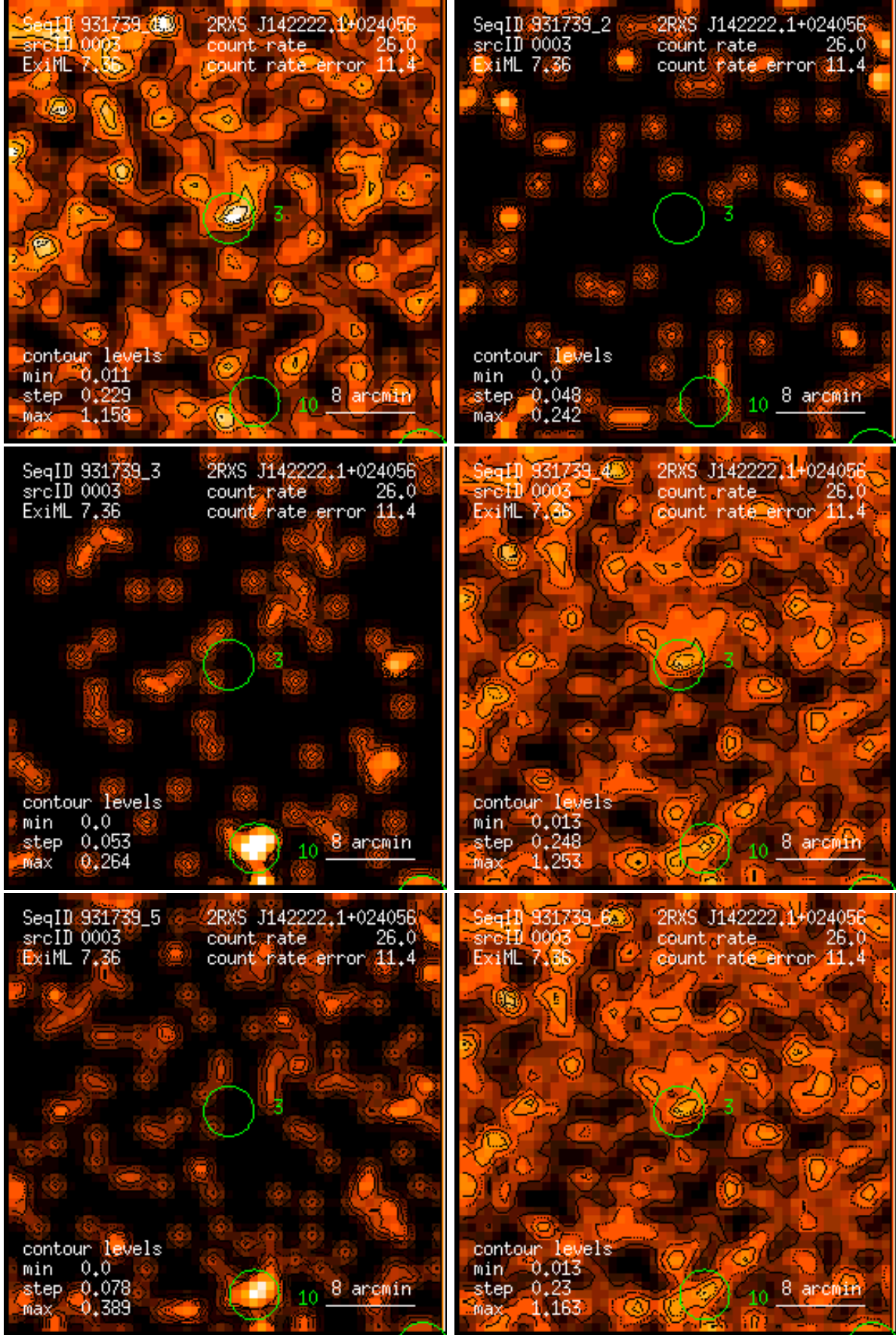
Figure 3: RASS 931739: detection 0003: band rate images, Gaussian filter: (1) PSPC channels 11 – 41, (2) 52 – 90, (3) 91 – 201, (4) 11 – 235, (5) 52 – 201, (6) 11 – 201. Broad band rates in counts/ks. Band rate contour levels in counts/ks/arcmin 2 .
