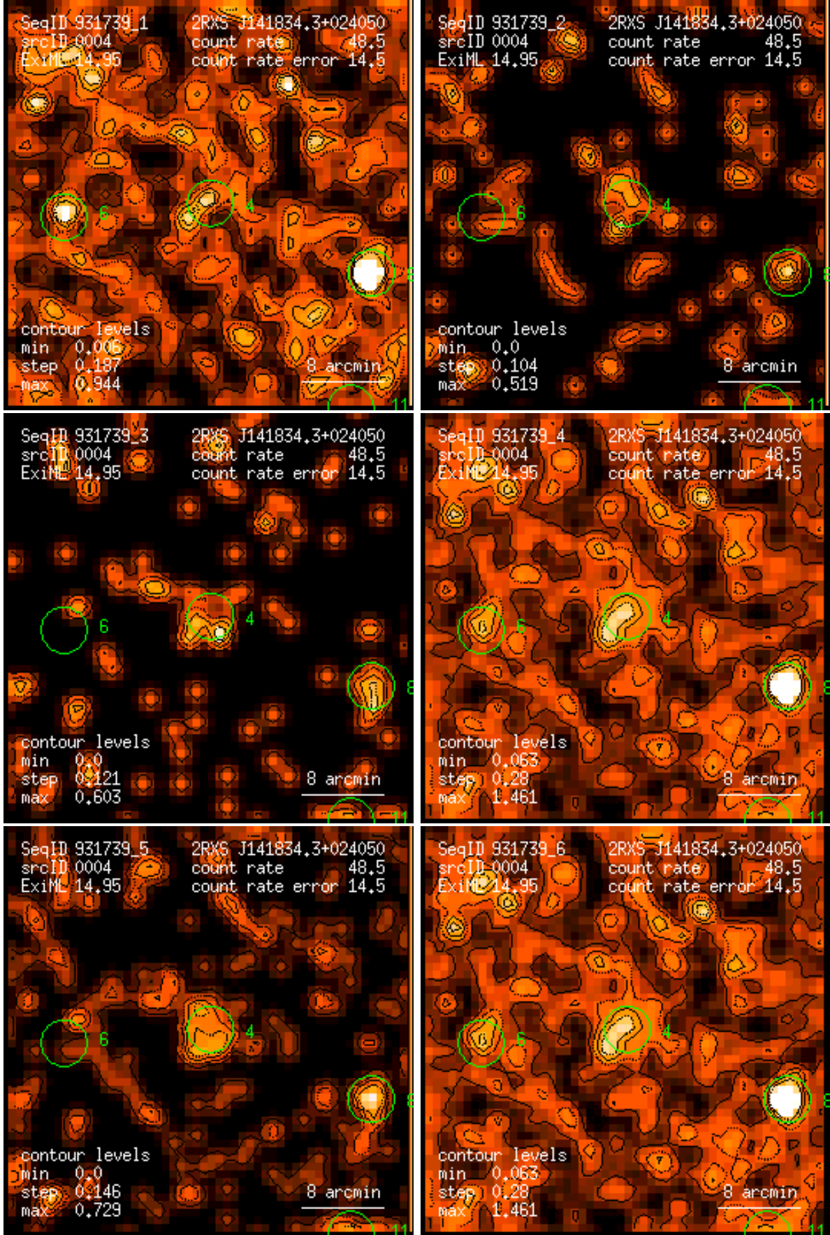
Figure 4: RASS 931739: detection 0004: band rate images, Gaussian filter: (1) PSPC channels 11 – 41, (2) 52 – 90, (3) 91 – 201, (4) 11 – 235, (5) 52 – 201, (6) 11 – 201. Broad band rates in counts/ks. Band rate contour levels in counts/ks/arcmin 2 .
