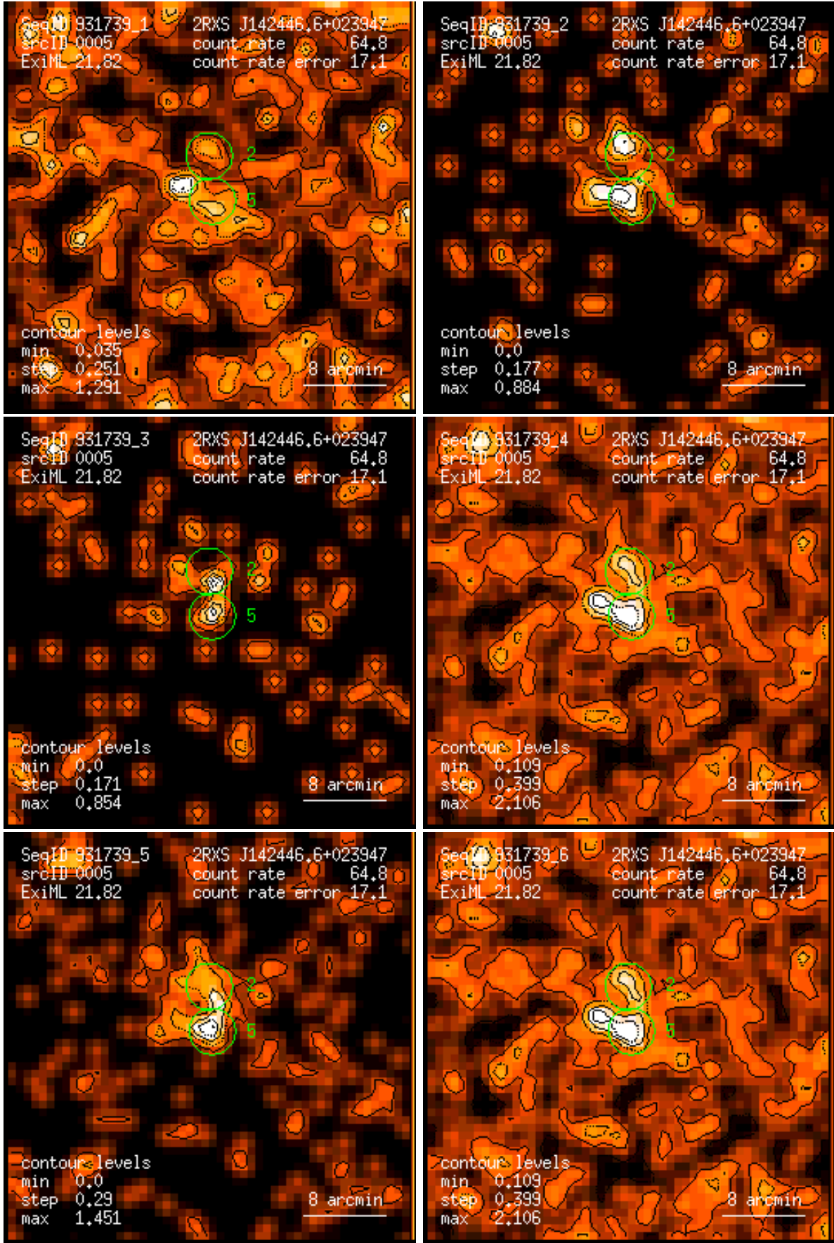
Figure 5: RASS 931739: detection 0005: band rate images, Gaussian filter: (1) PSPC channels 11 – 41, (2) 52 – 90, (3) 91 – 201, (4) 11 – 235, (5) 52 – 201, (6) 11 – 201. Broad band rates in counts/ks. Band rate contour levels in counts/ks/arcmin 2 .
