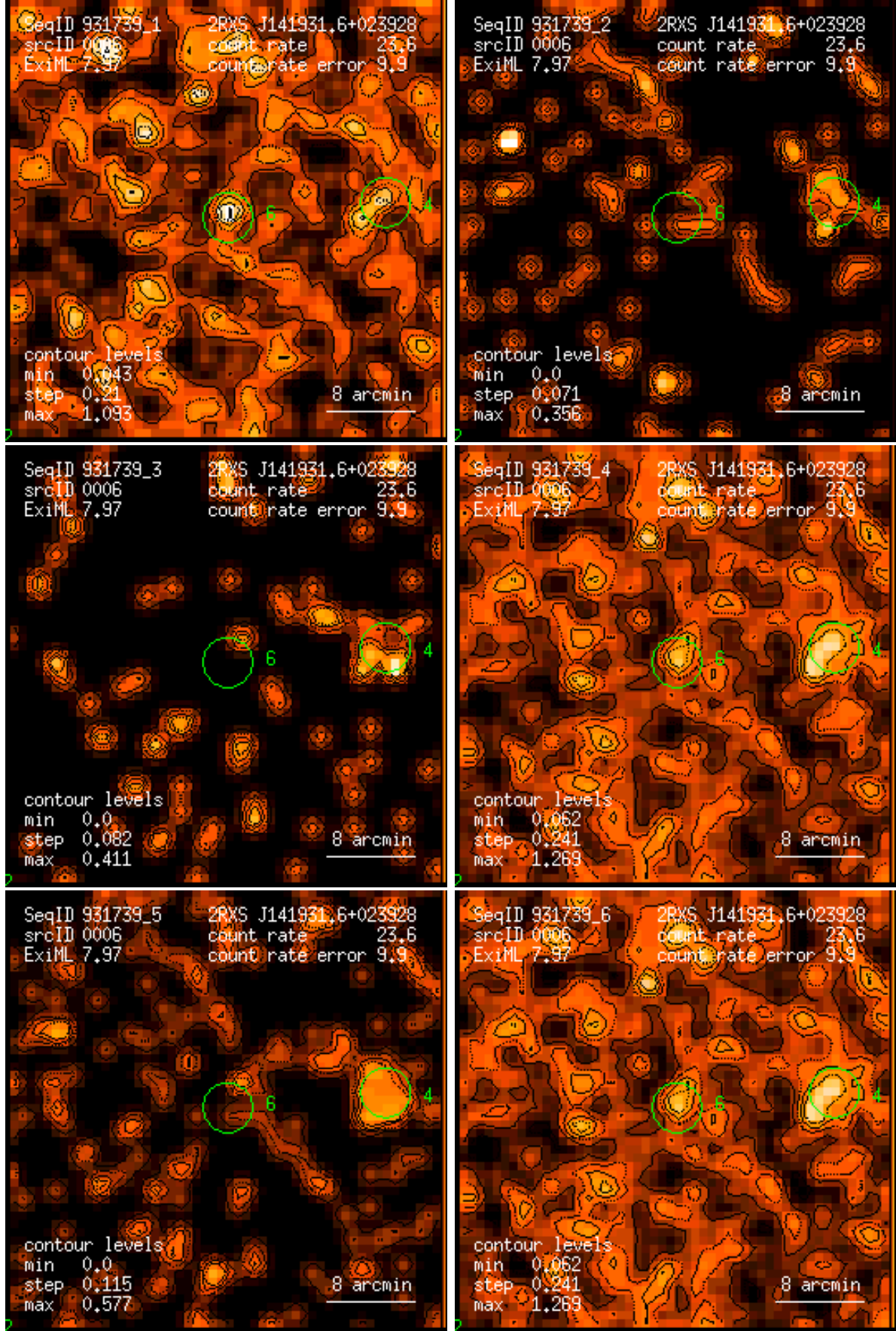
Figure 6: RASS 931739: detection 0006: band rate images, Gaussian filter: (1) PSPC channels 11 – 41, (2) 52 – 90, (3) 91 – 201, (4) 11 – 235, (5) 52 – 201, (6) 11 – 201. Broad band rates in counts/ks. Band rate contour levels in counts/ks/arcmin 2 .
