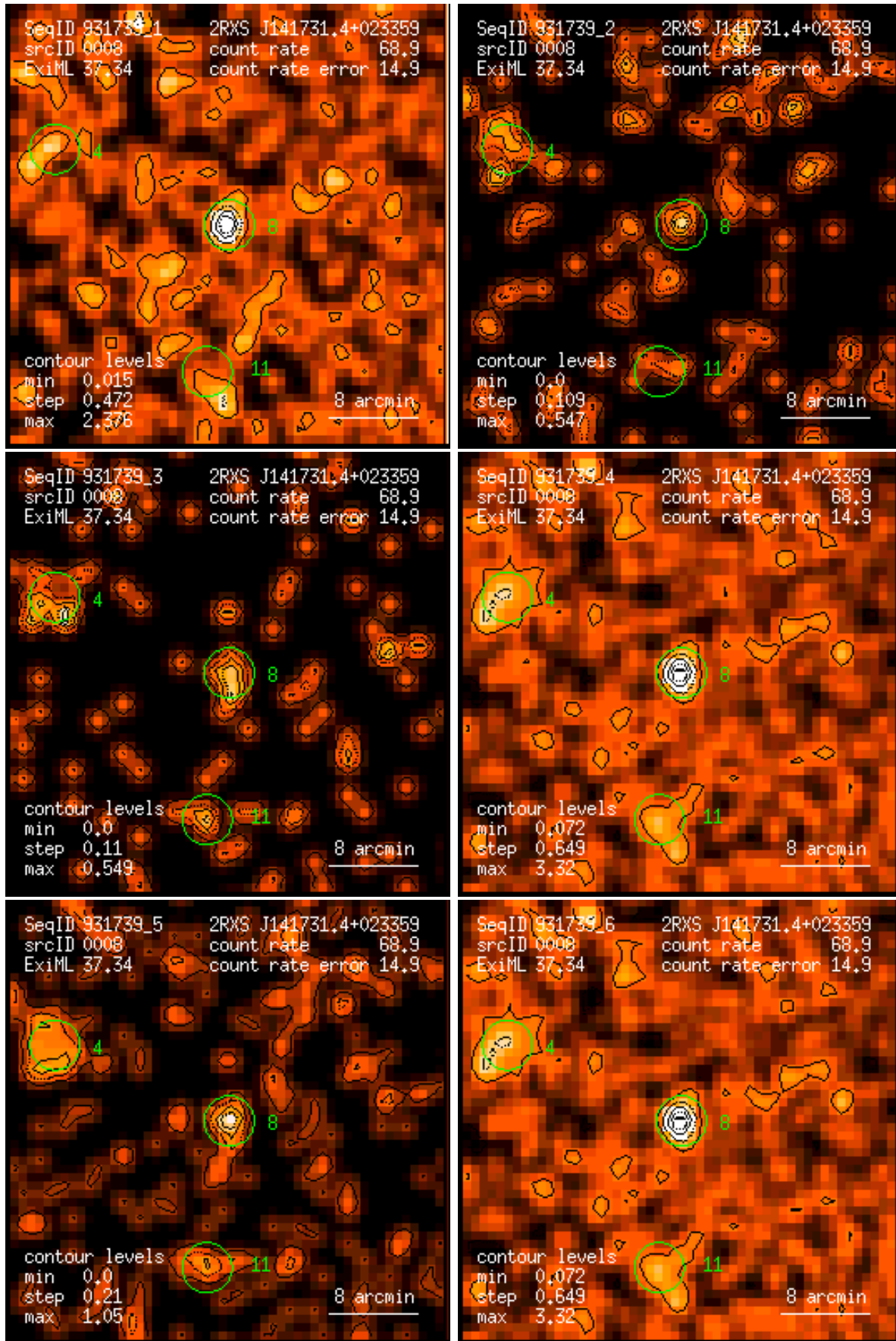
Figure 8: RASS 931739: detection 0008: band rate images, Gaussian filter: (1) PSPC channels 11 – 41, (2) 52 – 90, (3) 91 – 201, (4) 11 – 235, (5) 52 – 201, (6) 11 – 201. Broad band rates in counts/ks. Band rate contour levels in counts/ks/arcmin 2 .
